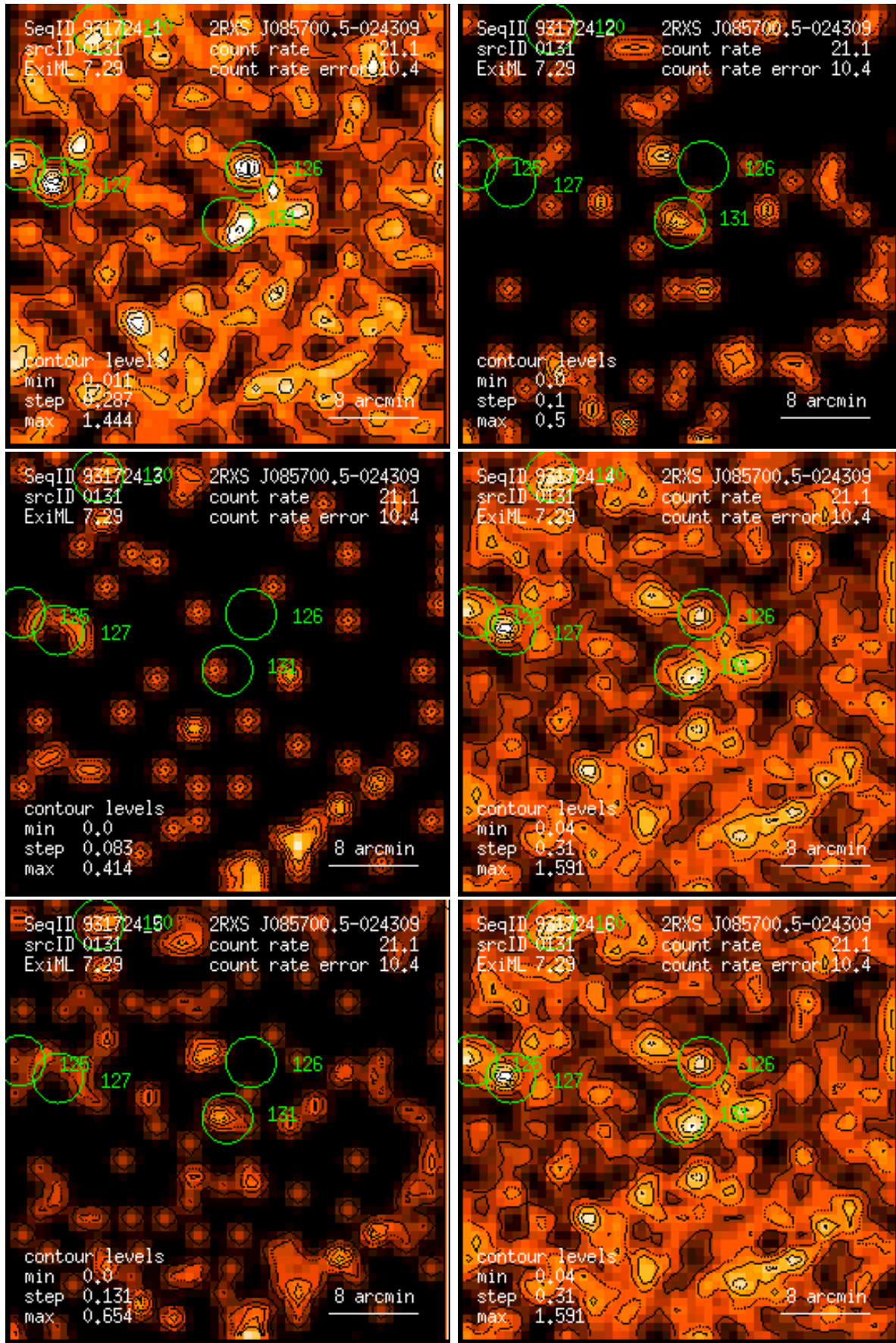
Figure 131: RASS 931724: detection 0131: band rate images, Gaussian filter: (1) PSPC channels 11 – 41, (2) 52 – 90, (3) 91 – 201, (4) 11 – 235, (5) 52 – 201, (6) 11 – 201. Broad band rates in counts/ks. Band rate contour levels in counts/ks/arcmin 2 .
