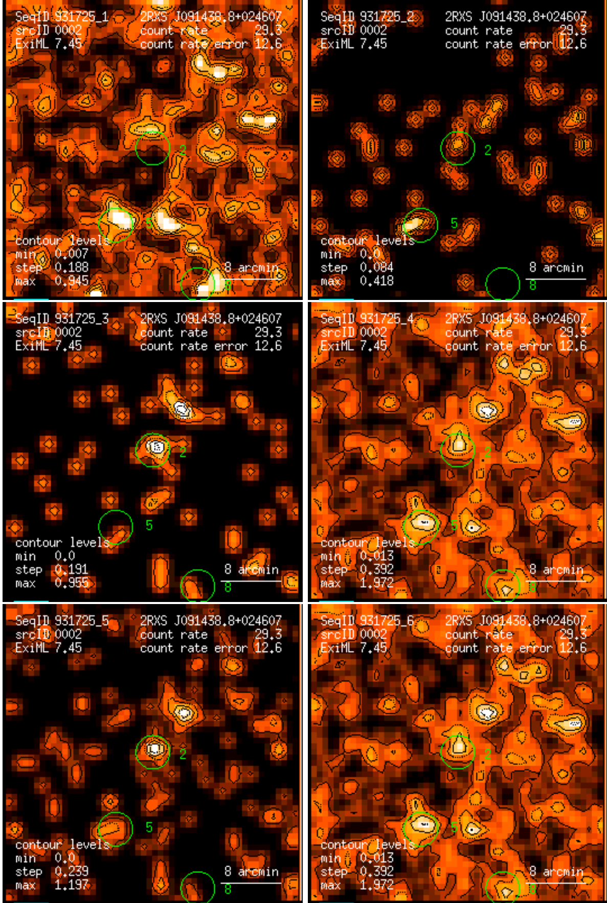
Figure 2: RASS 931725: detection 0002: band rate images, Gaussian filter: (1) PSPC channels 11 – 41, (2) 52 – 90, (3) 91 – 201, (4) 11 – 235, (5) 52 – 201, (6) 11 – 201. Broad band rates in counts/ks. Band rate contour levels in counts/ks/arcmin 2 .
