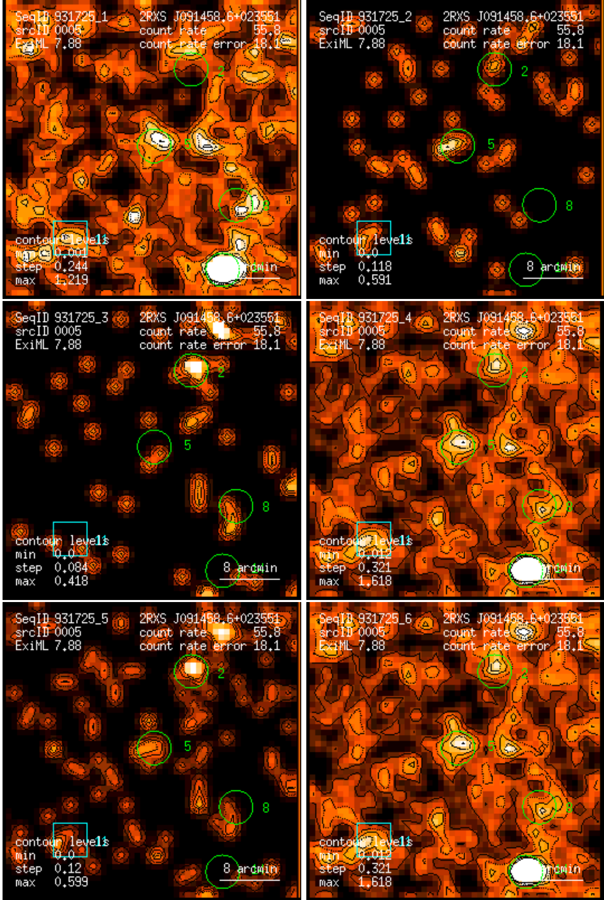
Figure 5: RASS 931725: detection 0005: band rate images, Gaussian filter: (1) PSPC channels 11 – 41, (2) 52 – 90, (3) 91 – 201, (4) 11 – 235, (5) 52 – 201, (6) 11 – 201. Broad band rates in counts/ks. Band rate contour levels in counts/ks/arcmin 2 .
