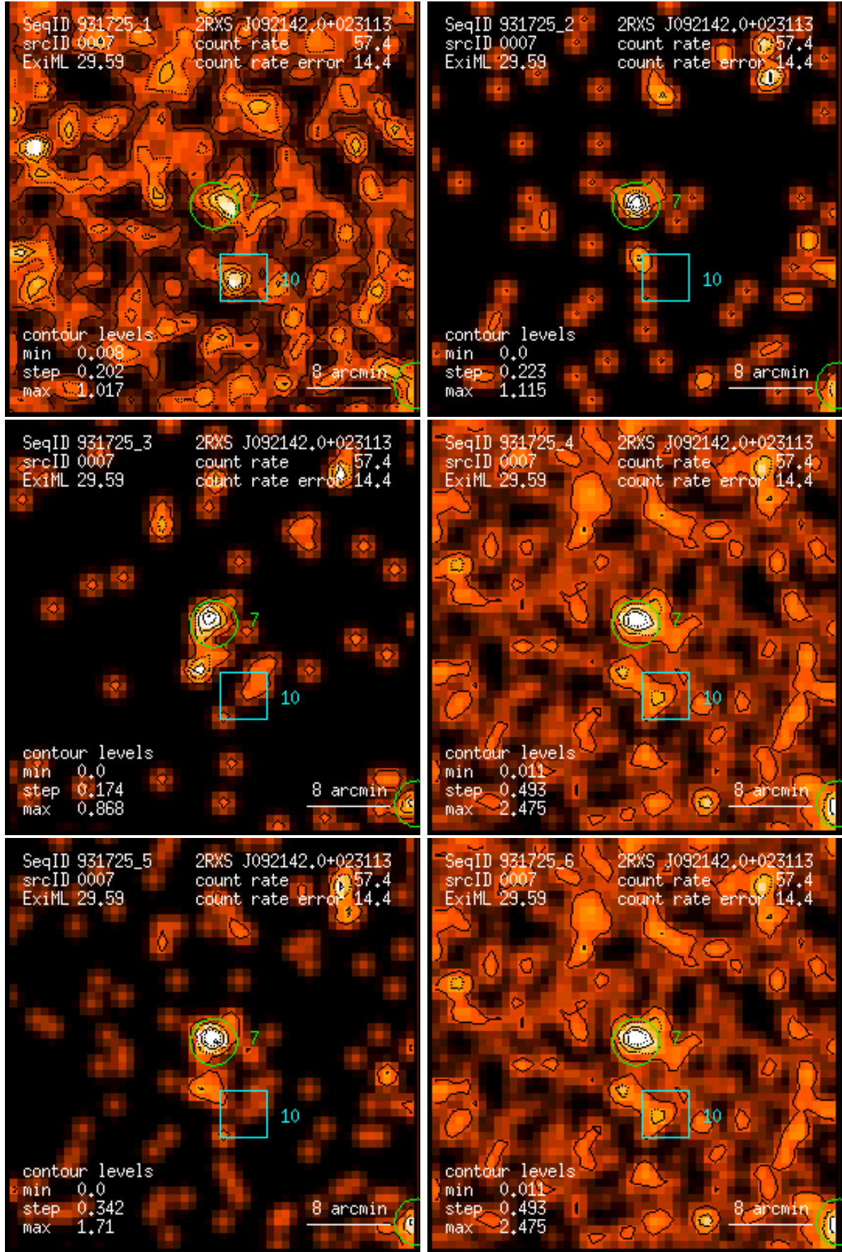
Figure 7: RASS 931725: detection 0007: band rate images, Gaussian filter: (1) PSPC channels 11 – 41, (2) 52 – 90, (3) 91 – 201, (4) 11 – 235, (5) 52 – 201, (6) 11 – 201. Broad band rates in counts/ks. Band rate contour levels in counts/ks/arcmin 2 .
