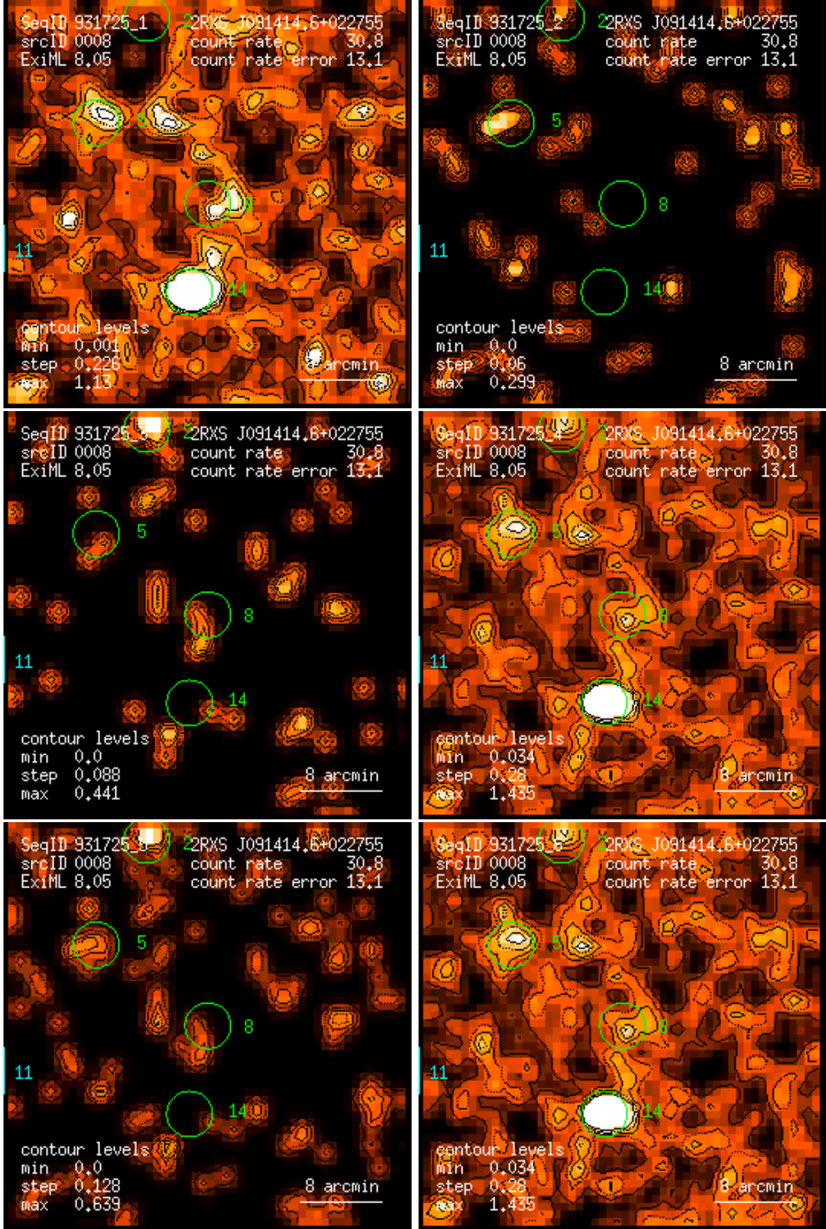
Figure 8: RASS 931725: detection 0008: band rate images, Gaussian filter: (1) PSPC channels 11 – 41, (2) 52 – 90, (3) 91 – 201, (4) 11 – 235, (5) 52 – 201, (6) 11 – 201. Broad band rates in counts/ks. Band rate contour levels in counts/ks/arcmin 2 .
