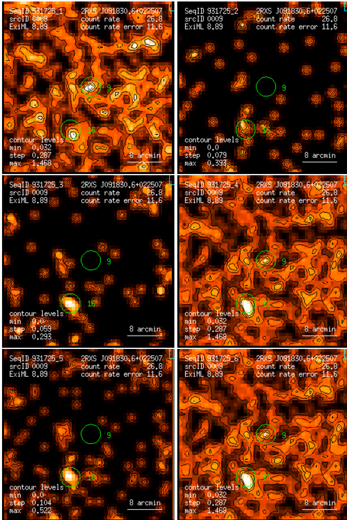
Figure 9: RASS 931725: detection 0009: band rate images, Gaussian filter: (1) PSPC channels 11 – 41, (2) 52 – 90, (3) 91 – 201, (4) 11 – 235, (5) 52 – 201, (6) 11 – 201. Broad band rates in counts/ks. Band rate contour levels in counts/ks/arcmin 2 .
