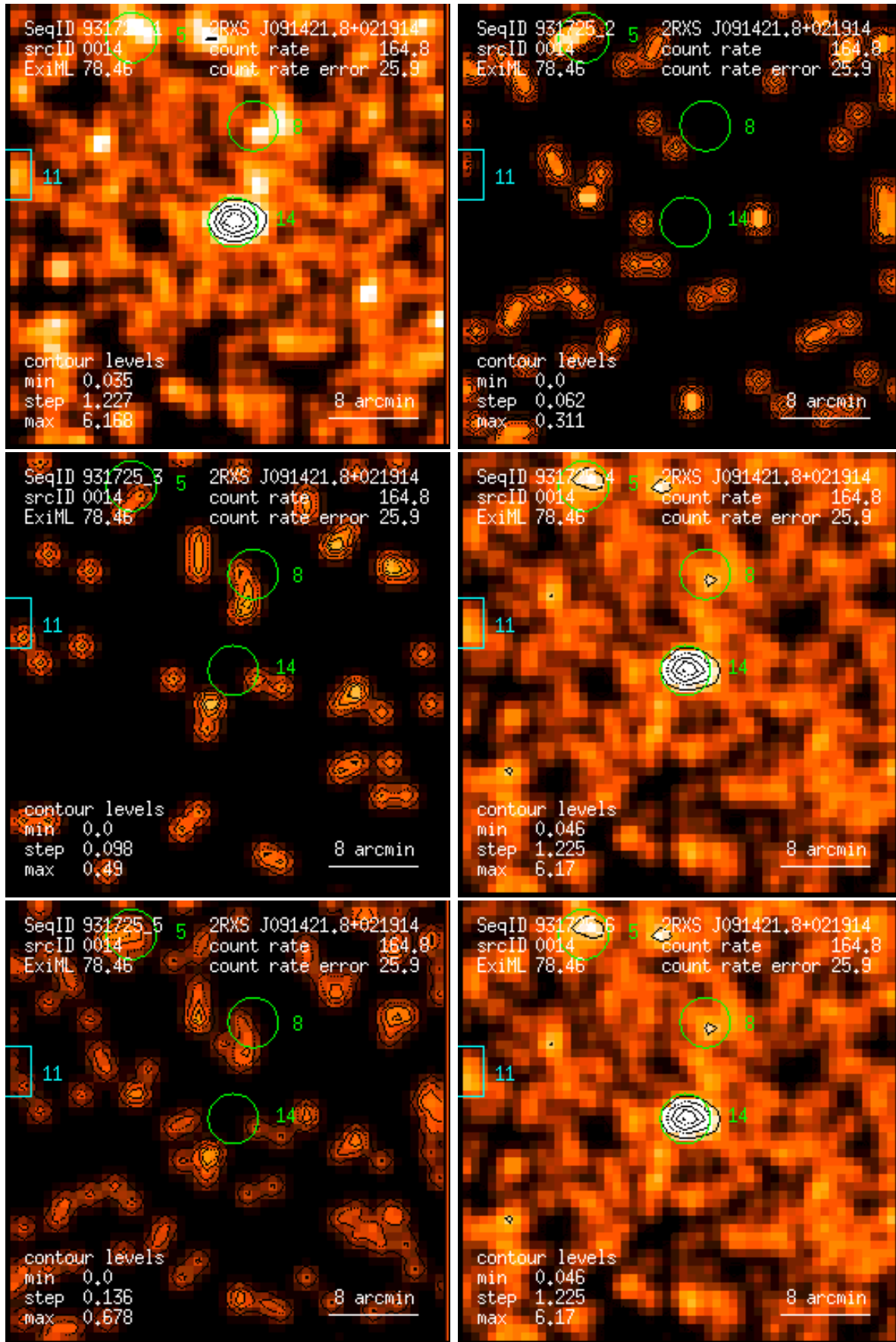
Figure 14: RASS 931725: detection 0014: band rate images, Gaussian filter: (1) PSPC channels 11 – 41, (2) 52 – 90, (3) 91 – 201, (4) 11 – 235, (5) 52 – 201, (6) 11 – 201. Broad band rates in counts/ks. Band rate contour levels in counts/ks/arcmin 2 .
