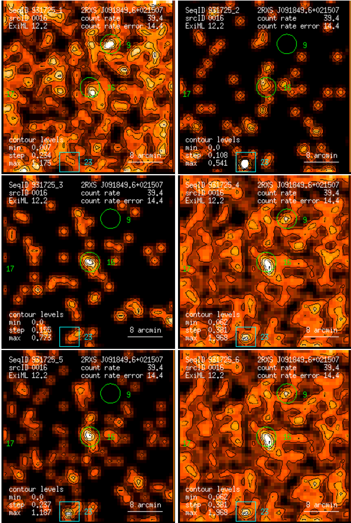
Figure 16: RASS 931725: detection 0016: band rate images, Gaussian filter: (1) PSPC channels 11 – 41, (2) 52 – 90, (3) 91 – 201, (4) 11 – 235, (5) 52 – 201, (6) 11 – 201. Broad band rates in counts/ks. Band rate contour levels in counts/ks/arcmin 2 .
