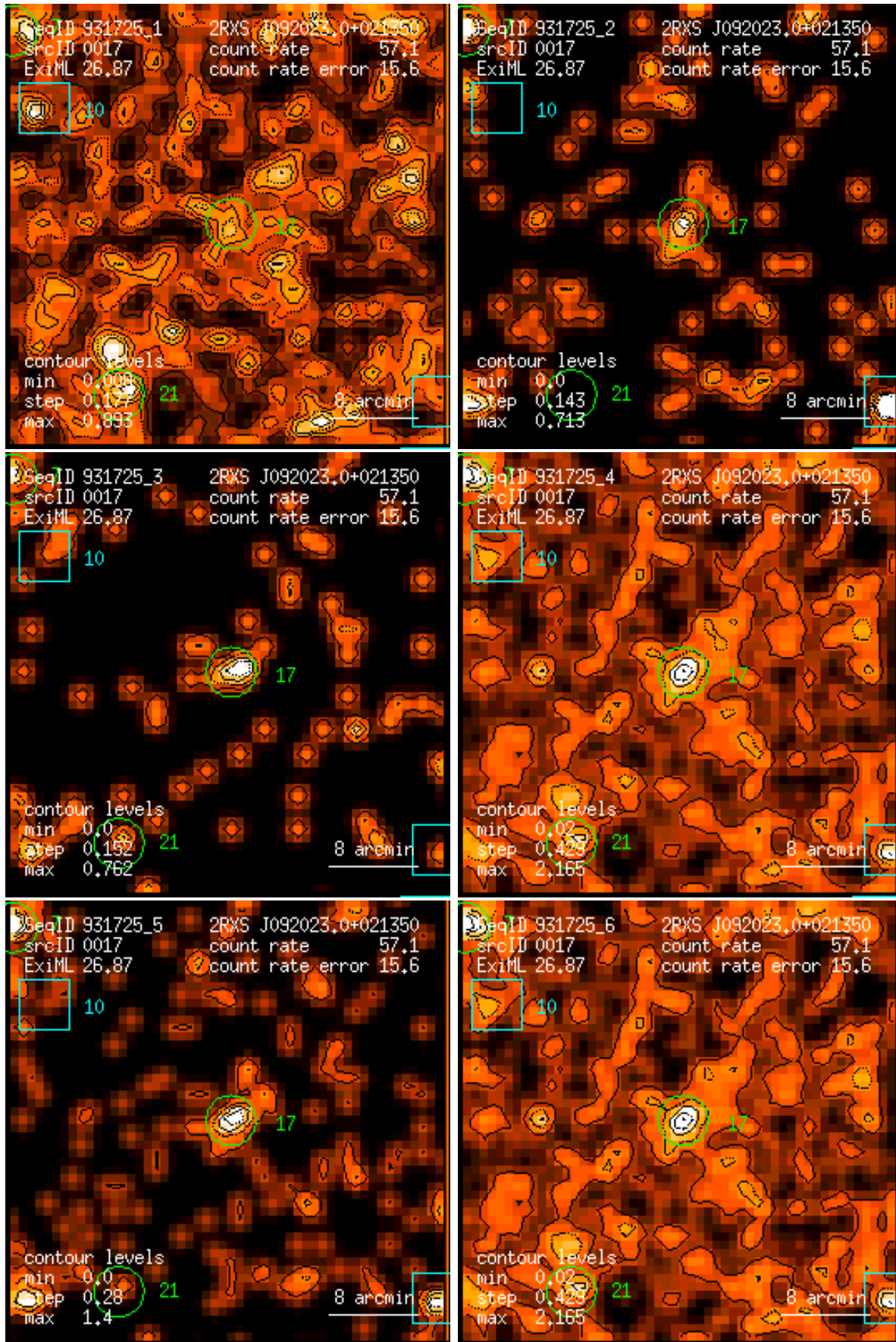
Figure 17: RASS 931725: detection 0017: band rate images, Gaussian filter: (1) PSPC channels 11 – 41, (2) 52 – 90, (3) 91 – 201, (4) 11 – 235, (5) 52 – 201, (6) 11 – 201. Broad band rates in counts/ks. Band rate contour levels in counts/ks/arcmin 2 .
