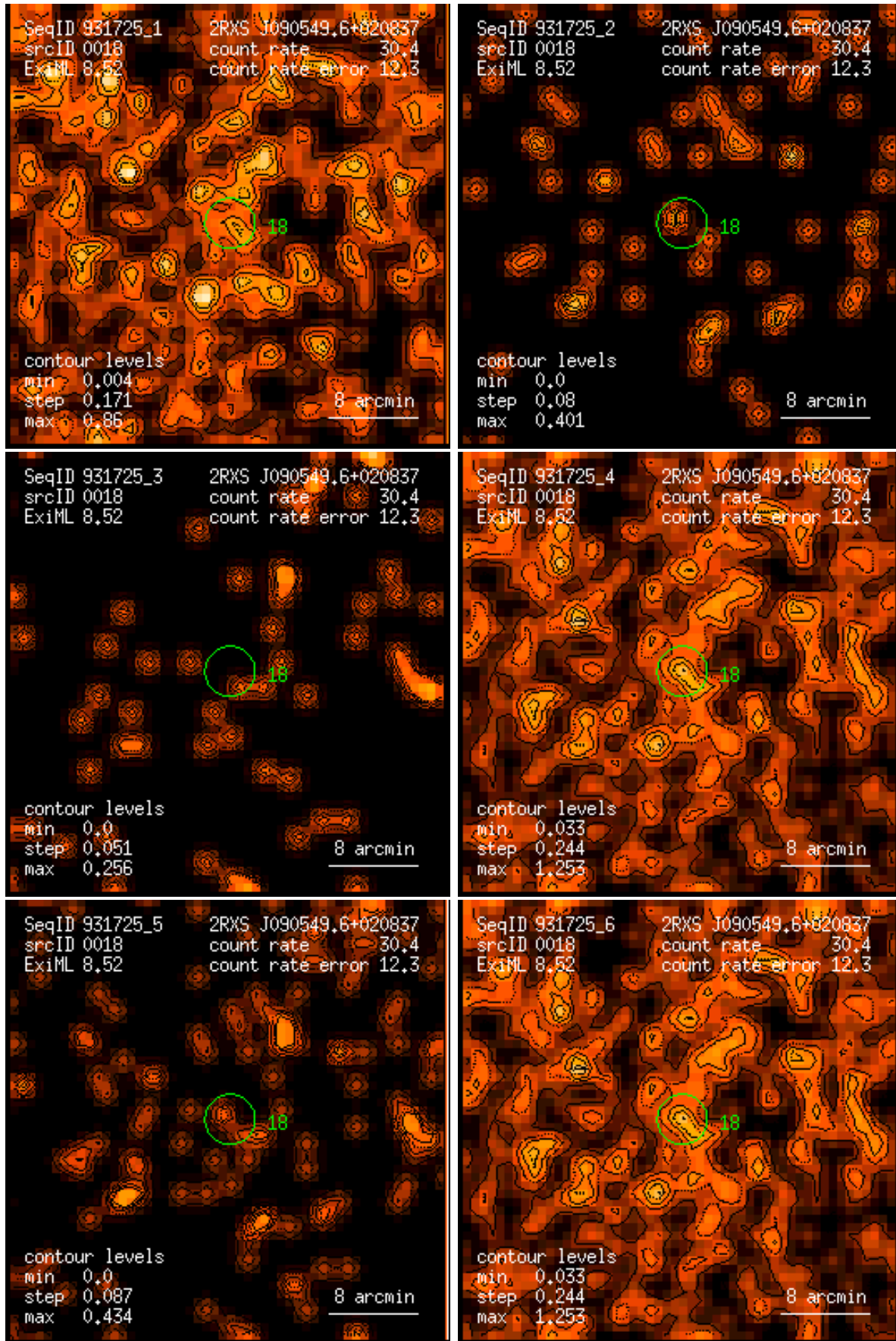
Figure 18: RASS 931725: detection 0018: band rate images, Gaussian filter: (1) PSPC channels 11 – 41, (2) 52 – 90, (3) 91 – 201, (4) 11 – 235, (5) 52 – 201, (6) 11 – 201. Broad band rates in counts/ks. Band rate contour levels in counts/ks/arcmin 2 .
