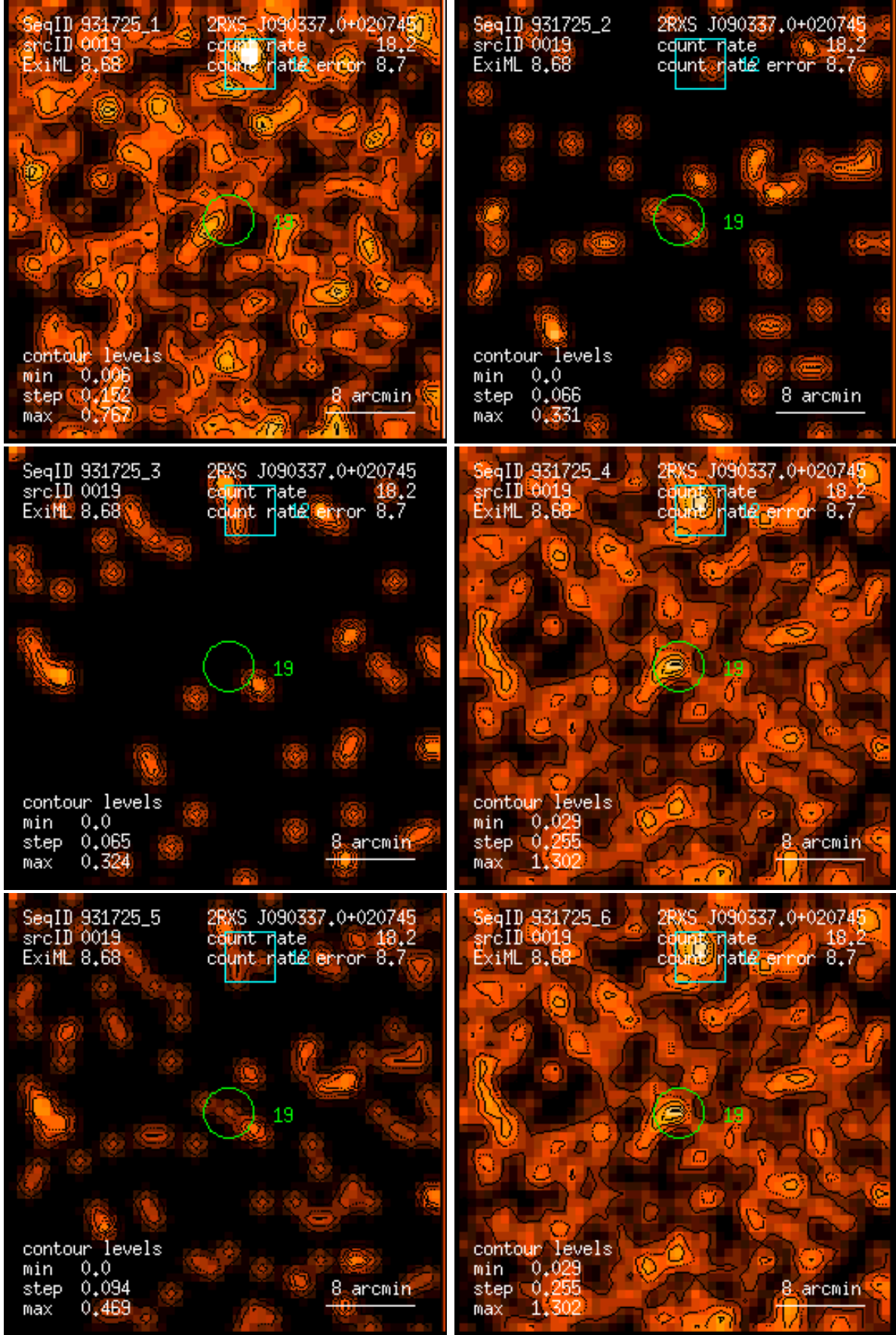
Figure 19: RASS 931725: detection 0019: band rate images, Gaussian filter: (1) PSPC channels 11 – 41, (2) 52 – 90, (3) 91 – 201, (4) 11 – 235, (5) 52 – 201, (6) 11 – 201. Broad band rates in counts/ks. Band rate contour levels in counts/ks/arcmin 2 .
