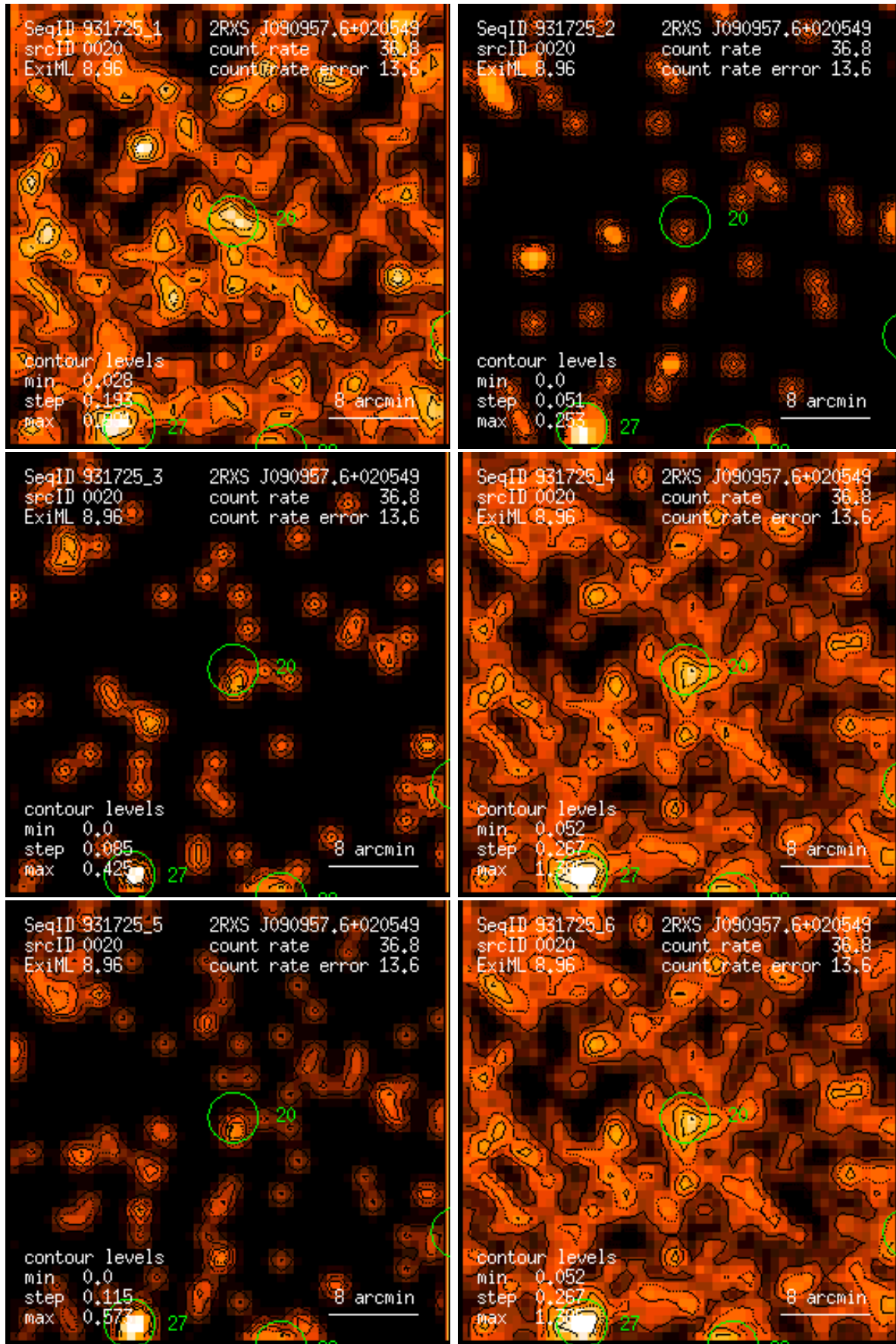
Figure 20: RASS 931725: detection 0020: band rate images, Gaussian filter: (1) PSPC channels 11 – 41, (2) 52 – 90, (3) 91 – 201, (4) 11 – 235, (5) 52 – 201, (6) 11 – 201. Broad band rates in counts/ks. Band rate contour levels in counts/ks/arcmin 2 .
