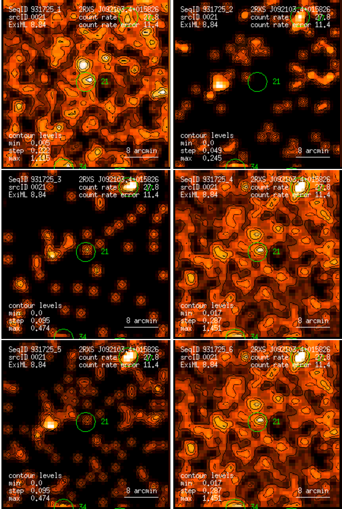
Figure 21: RASS 931725: detection 0021: band rate images, Gaussian filter: (1) PSPC channels 11 – 41, (2) 52 – 90, (3) 91 – 201, (4) 11 – 235, (5) 52 – 201, (6) 11 – 201. Broad band rates in counts/ks. Band rate contour levels in counts/ks/arcmin 2 .
