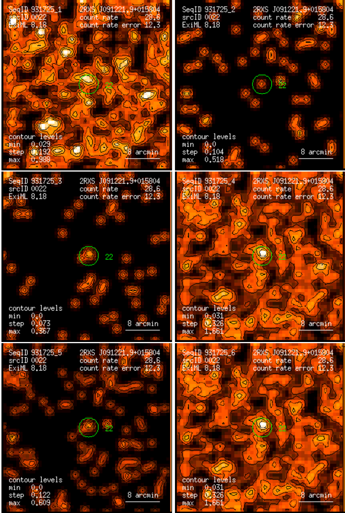
Figure 22: RASS 931725: detection 0022: band rate images, Gaussian filter: (1) PSPC channels 11 – 41, (2) 52 – 90, (3) 91 – 201, (4) 11 – 235, (5) 52 – 201, (6) 11 – 201. Broad band rates in counts/ks. Band rate contour levels in counts/ks/arcmin 2 .
