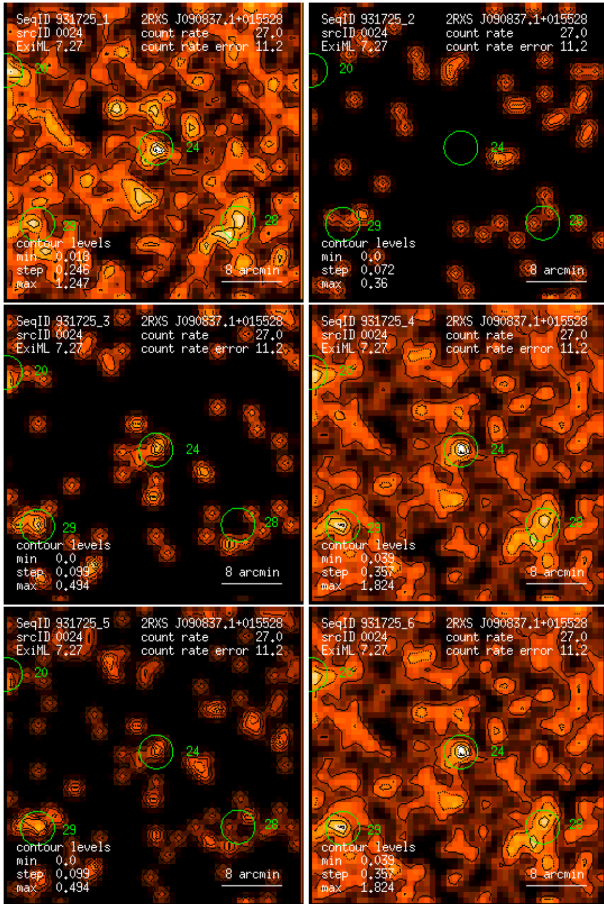
Figure 24: RASS 931725: detection 0024: band rate images, Gaussian filter: (1) PSPC channels 11 – 41, (2) 52 – 90, (3) 91 – 201, (4) 11 – 235, (5) 52 – 201, (6) 11 – 201. Broad band rates in counts/ks. Band rate contour levels in counts/ks/arcmin 2 .
