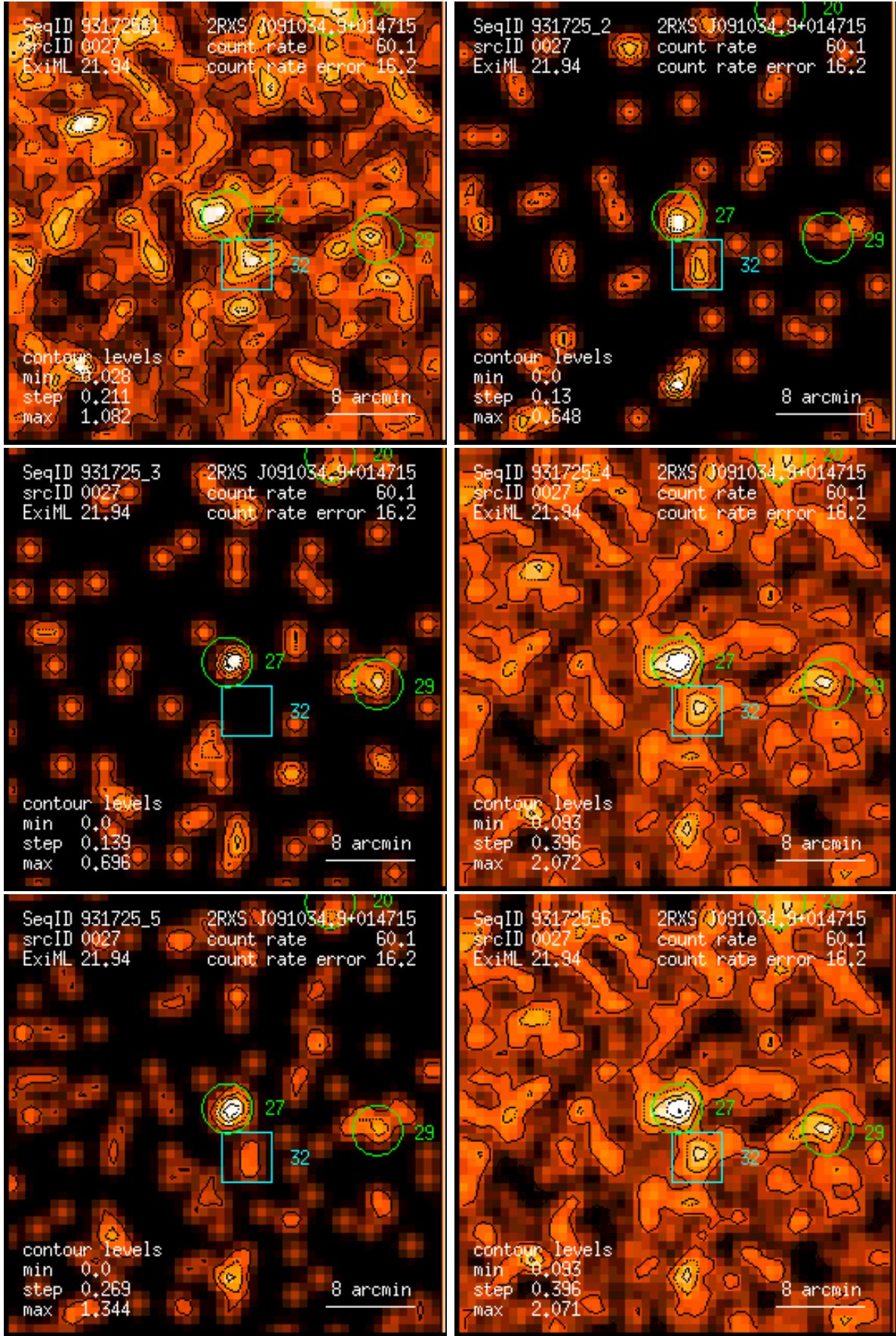
Figure 27: RASS 931725: detection 0027: band rate images, Gaussian filter: (1) PSPC channels 11 – 41, (2) 52 – 90, (3) 91 – 201, (4) 11 – 235, (5) 52 – 201, (6) 11 – 201. Broad band rates in counts/ks. Band rate contour levels in counts/ks/arcmin 2 .
