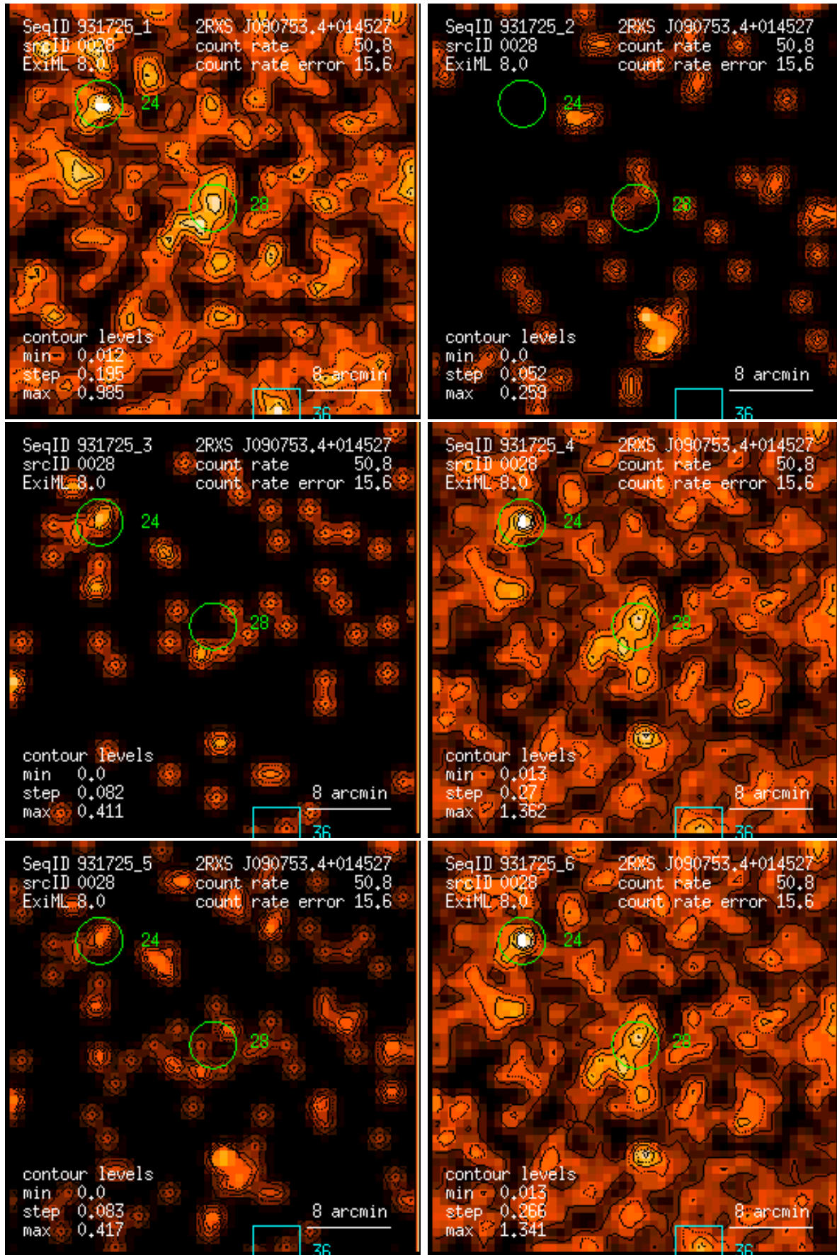
Figure 28: RASS 931725: detection 0028: band rate images, Gaussian filter: (1) PSPC channels 11 – 41, (2) 52 – 90, (3) 91 – 201, (4) 11 – 235, (5) 52 – 201, (6) 11 – 201. Broad band rates in counts/ks. Band rate contour levels in counts/ks/arcmin 2 .
