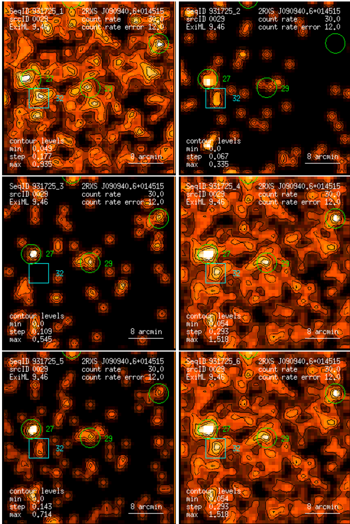
Figure 29: RASS 931725: detection 0029: band rate images, Gaussian filter: (1) PSPC channels 11 – 41, (2) 52 – 90, (3) 91 – 201, (4) 11 – 235, (5) 52 – 201, (6) 11 – 201. Broad band rates in counts/ks. Band rate contour levels in counts/ks/arcmin 2 .
