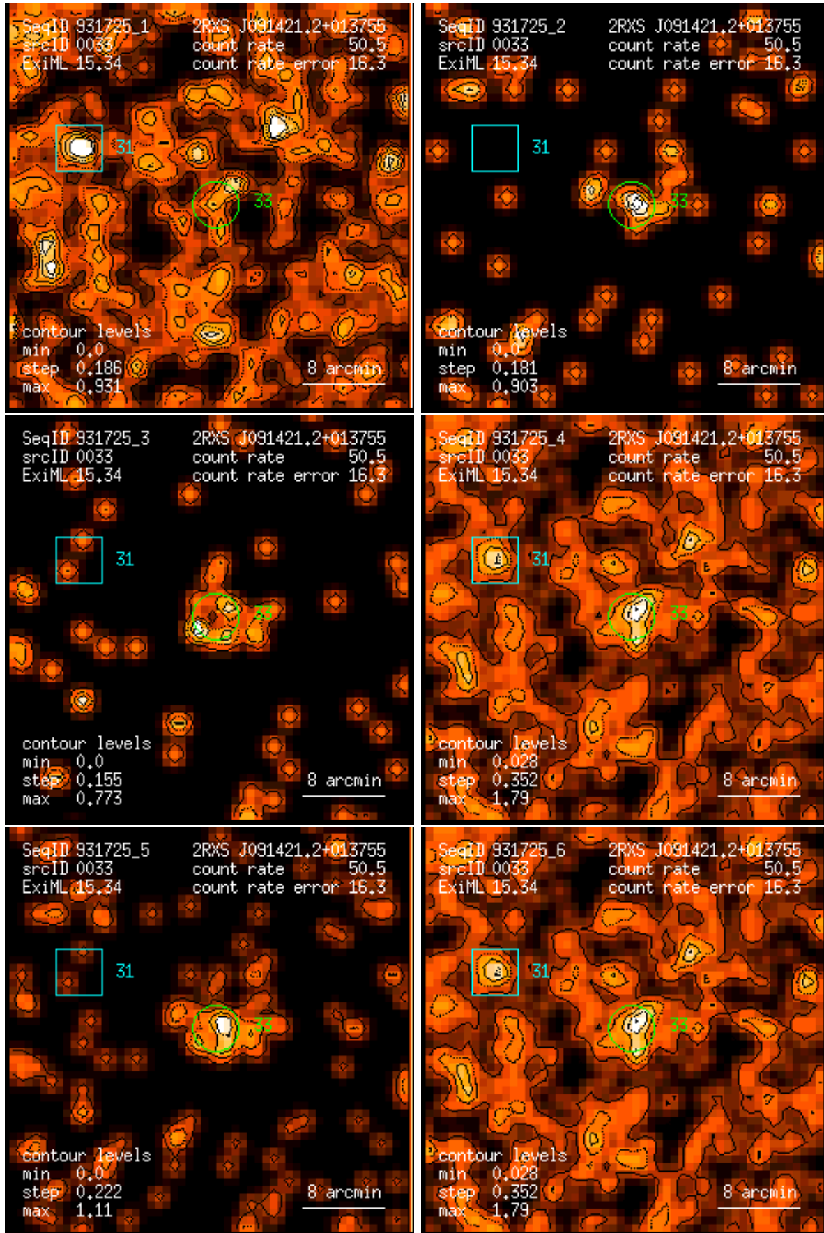
Figure 33: RASS 931725: detection 0033: band rate images, Gaussian filter: (1) PSPC channels 11 – 41, (2) 52 – 90, (3) 91 – 201, (4) 11 – 235, (5) 52 – 201, (6) 11 – 201. Broad band rates in counts/ks. Band rate contour levels in counts/ks/arcmin 2 .
