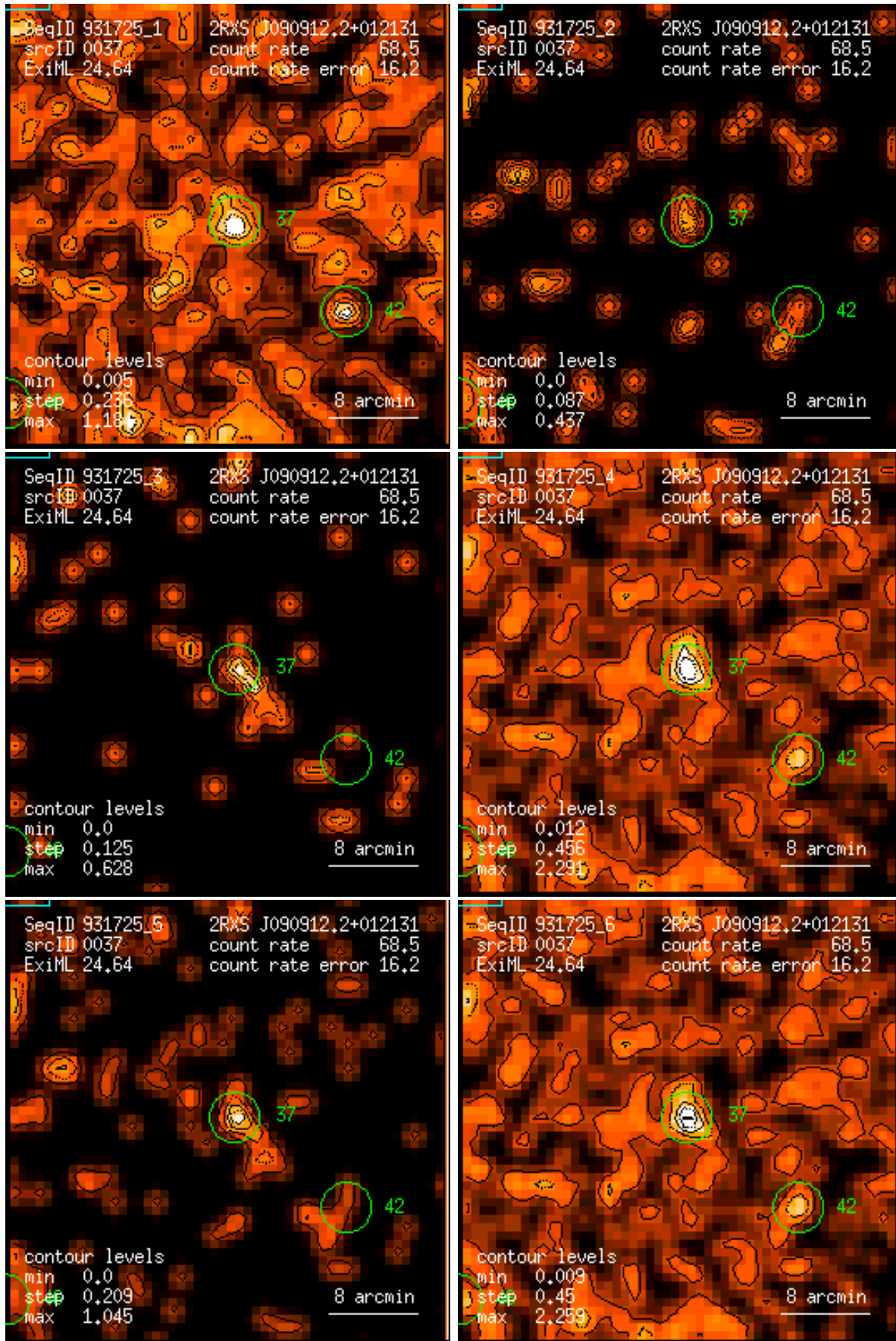
Figure 37: RASS 931725: detection 0037: band rate images, Gaussian filter: (1) PSPC channels 11 – 41, (2) 52 – 90, (3) 91 – 201, (4) 11 – 235, (5) 52 – 201, (6) 11 – 201. Broad band rates in counts/ks. Band rate contour levels in counts/ks/arcmin 2 .
