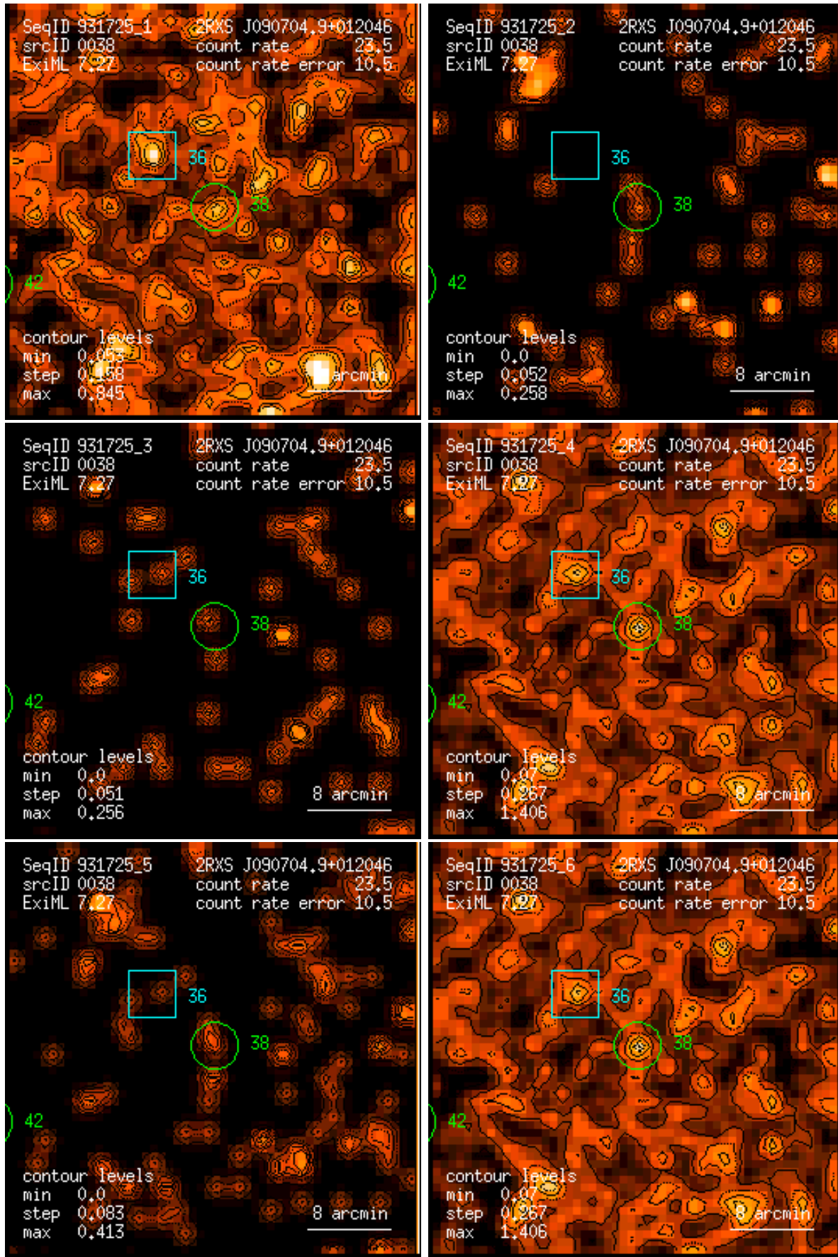
Figure 38: RASS 931725: detection 0038: band rate images, Gaussian filter: (1) PSPC channels 11 – 41, (2) 52 – 90, (3) 91 – 201, (4) 11 – 235, (5) 52 – 201, (6) 11 – 201. Broad band rates in counts/ks. Band rate contour levels in counts/ks/arcmin 2 .
