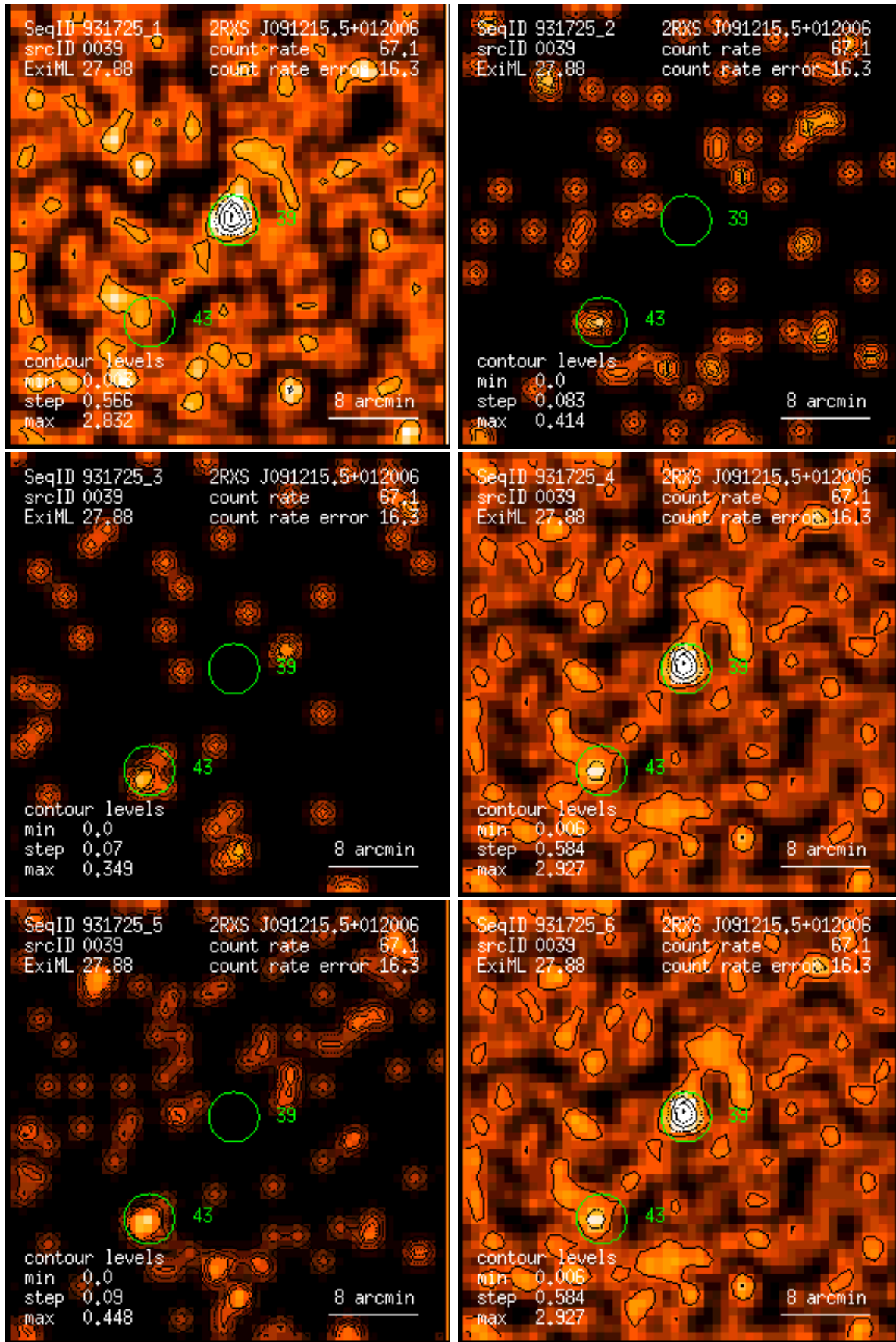
Figure 39: RASS 931725: detection 0039: band rate images, Gaussian filter: (1) PSPC channels 11 – 41, (2) 52 – 90, (3) 91 – 201, (4) 11 – 235, (5) 52 – 201, (6) 11 – 201. Broad band rates in counts/ks. Band rate contour levels in counts/ks/arcmin 2 .
