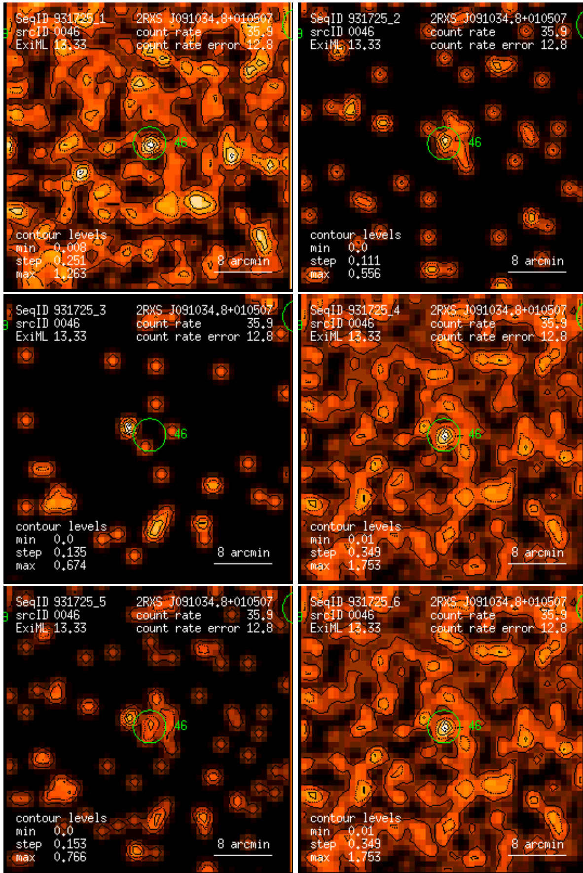
Figure 46: RASS 931725: detection 0046: band rate images, Gaussian filter: (1) PSPC channels 11 – 41, (2) 52 – 90, (3) 91 – 201, (4) 11 – 235, (5) 52 – 201, (6) 11 – 201. Broad band rates in counts/ks. Band rate contour levels in counts/ks/arcmin 2 .
