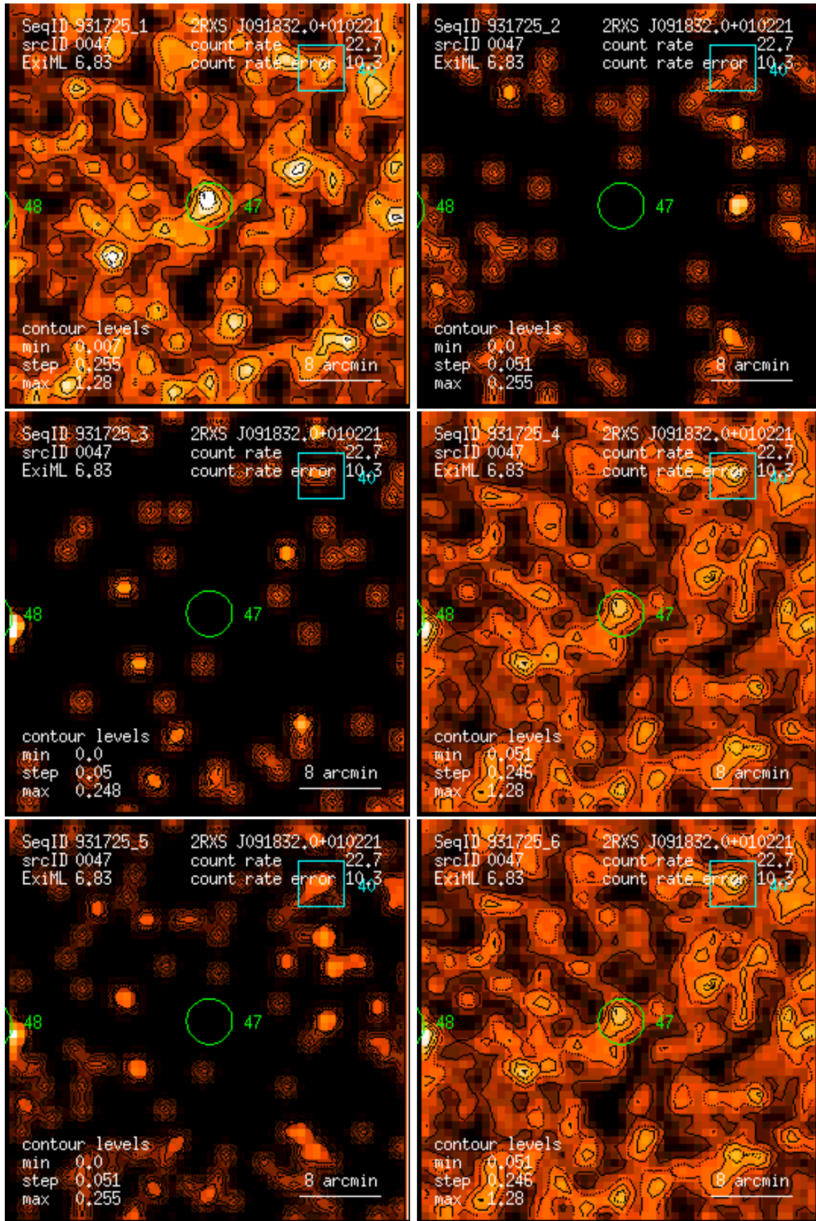
Figure 47: RASS 931725: detection 0047: band rate images, Gaussian filter: (1) PSPC channels 11 – 41, (2) 52 – 90, (3) 91 – 201, (4) 11 – 235, (5) 52 – 201, (6) 11 – 201. Broad band rates in counts/ks. Band rate contour levels in counts/ks/arcmin 2 .
