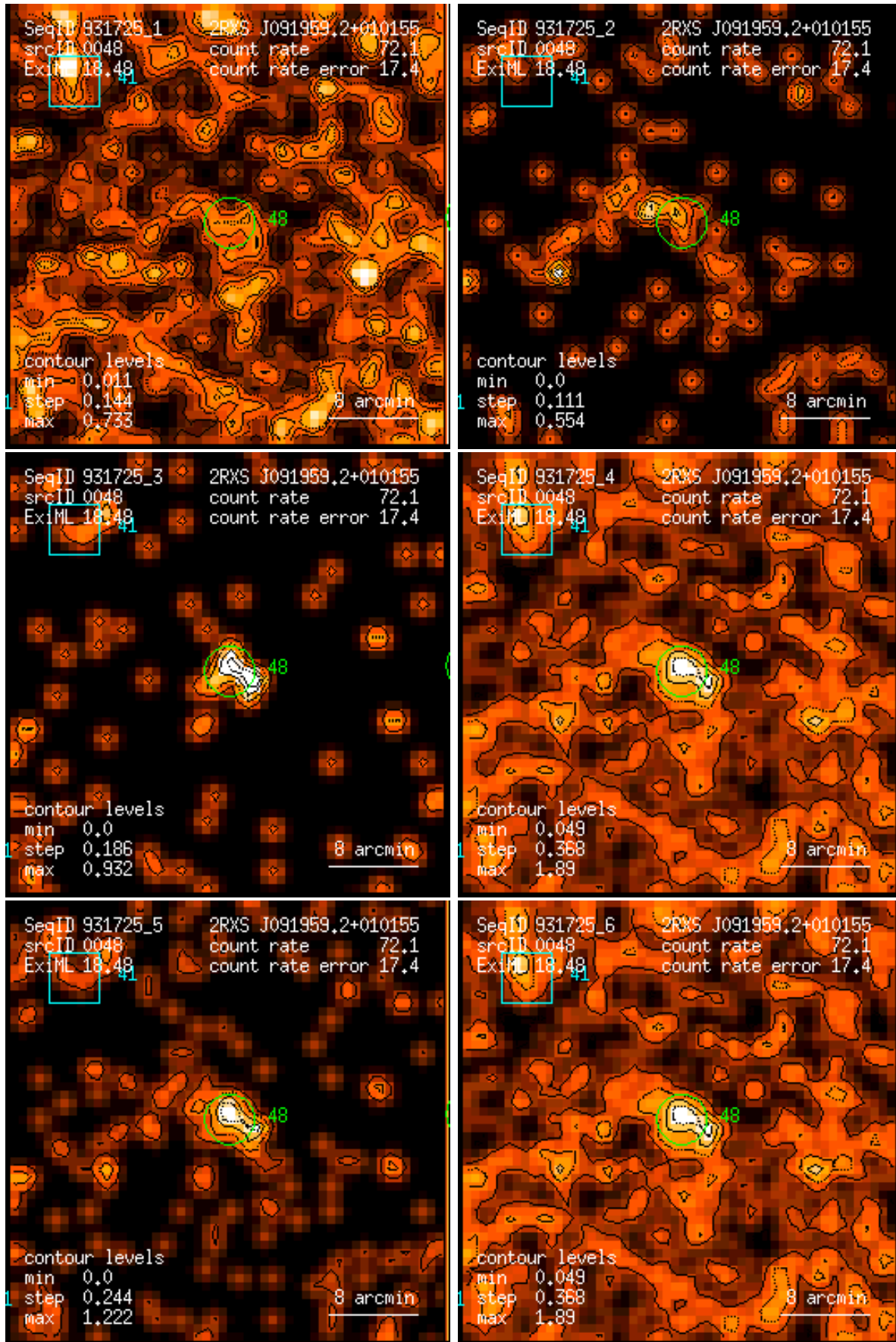
Figure 48: RASS 931725: detection 0048: band rate images, Gaussian filter: (1) PSPC channels 11 – 41, (2) 52 – 90, (3) 91 – 201, (4) 11 – 235, (5) 52 – 201, (6) 11 – 201. Broad band rates in counts/ks. Band rate contour levels in counts/ks/arcmin 2 .
