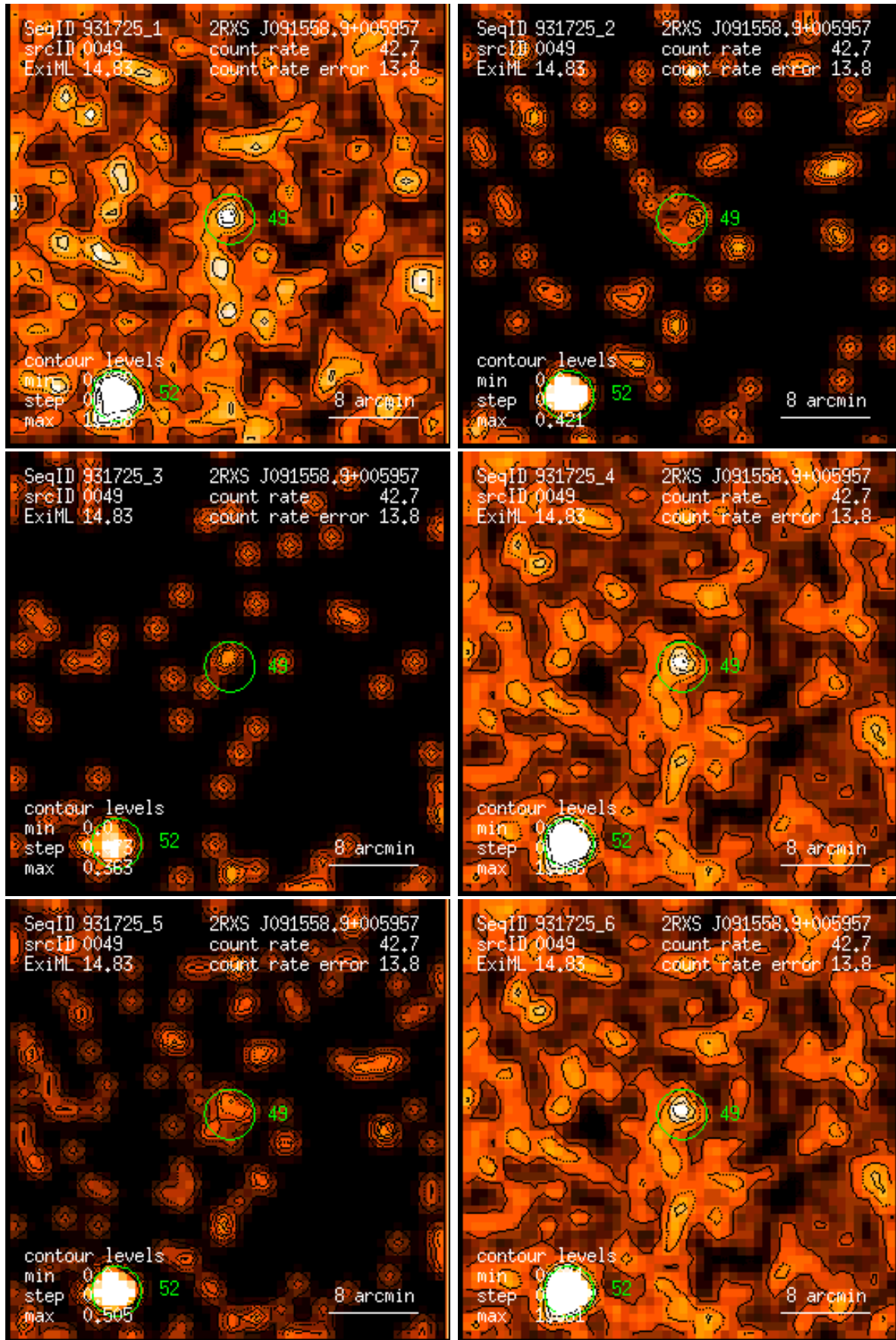
Figure 49: RASS 931725: detection 0049: band rate images, Gaussian filter: (1) PSPC channels 11 – 41, (2) 52 – 90, (3) 91 – 201, (4) 11 – 235, (5) 52 – 201, (6) 11 – 201. Broad band rates in counts/ks. Band rate contour levels in counts/ks/arcmin 2 .
