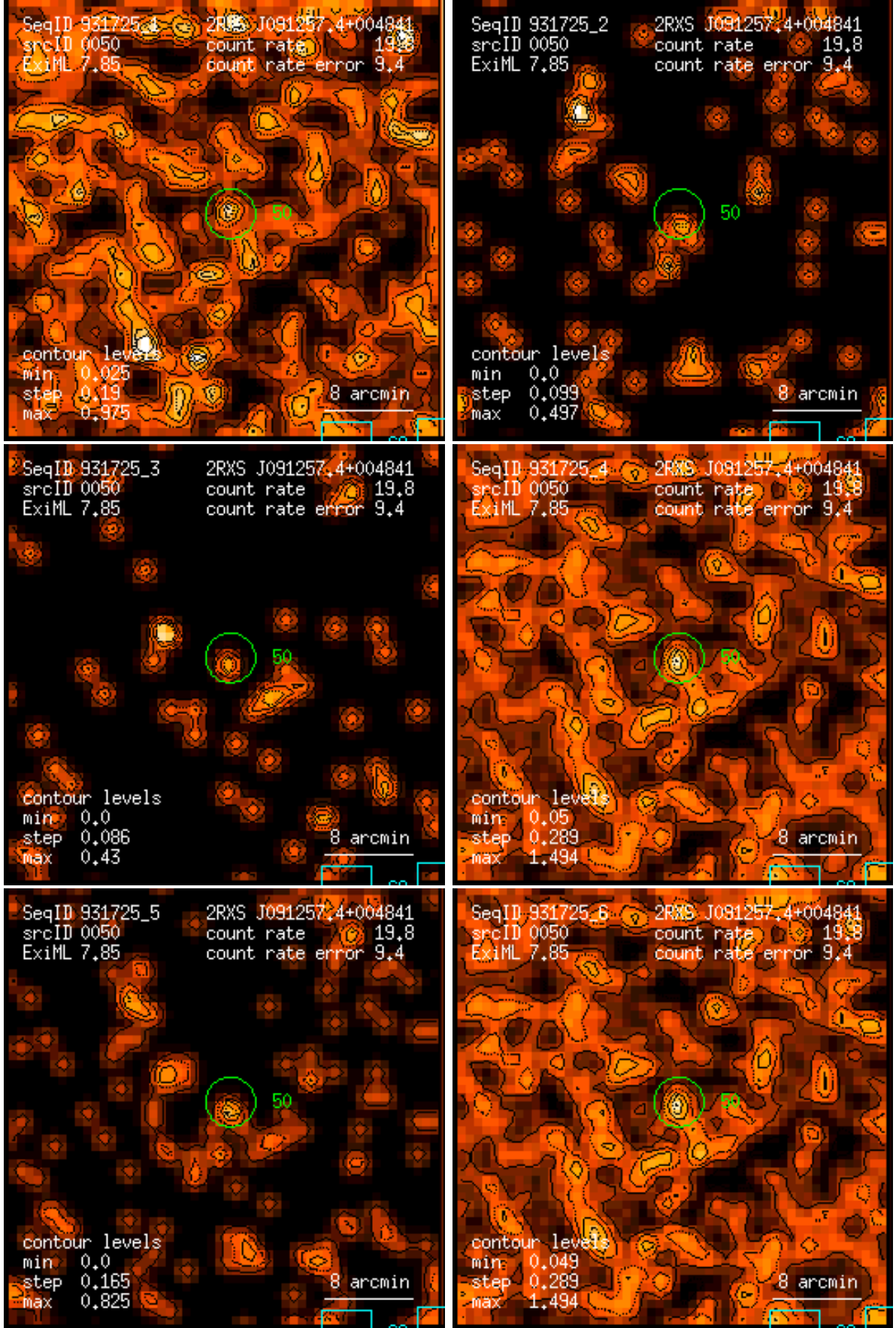
Figure 50: RASS 931725: detection 0050: band rate images, Gaussian filter: (1) PSPC channels 11 – 41, (2) 52 – 90, (3) 91 – 201, (4) 11 – 235, (5) 52 – 201, (6) 11 – 201. Broad band rates in counts/ks. Band rate contour levels in counts/ks/arcmin 2 .
