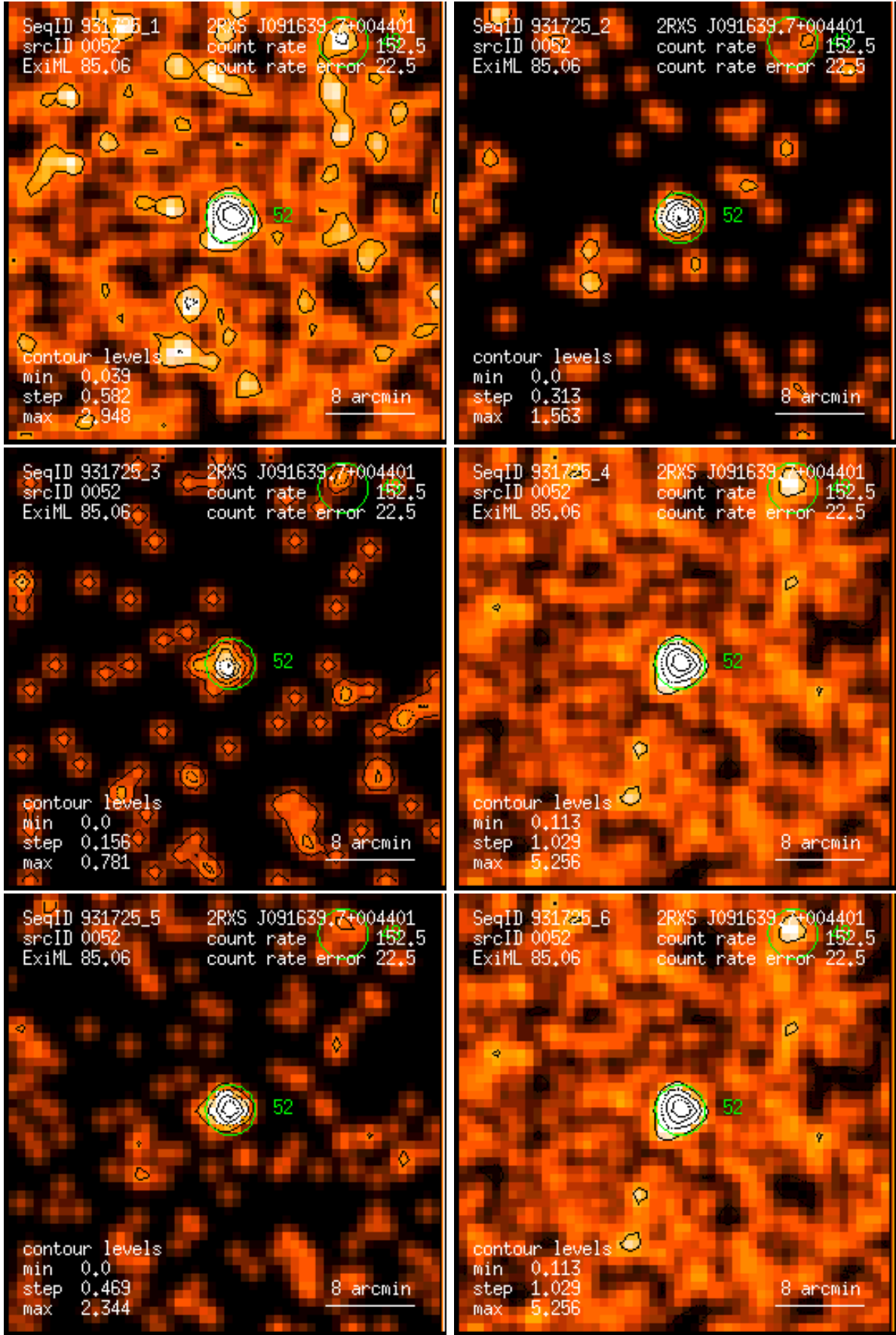
Figure 52: RASS 931725: detection 0052: band rate images, Gaussian filter: (1) PSPC channels 11 – 41, (2) 52 – 90, (3) 91 – 201, (4) 11 – 235, (5) 52 – 201, (6) 11 – 201. Broad band rates in counts/ks. Band rate contour levels in counts/ks/arcmin 2 .
