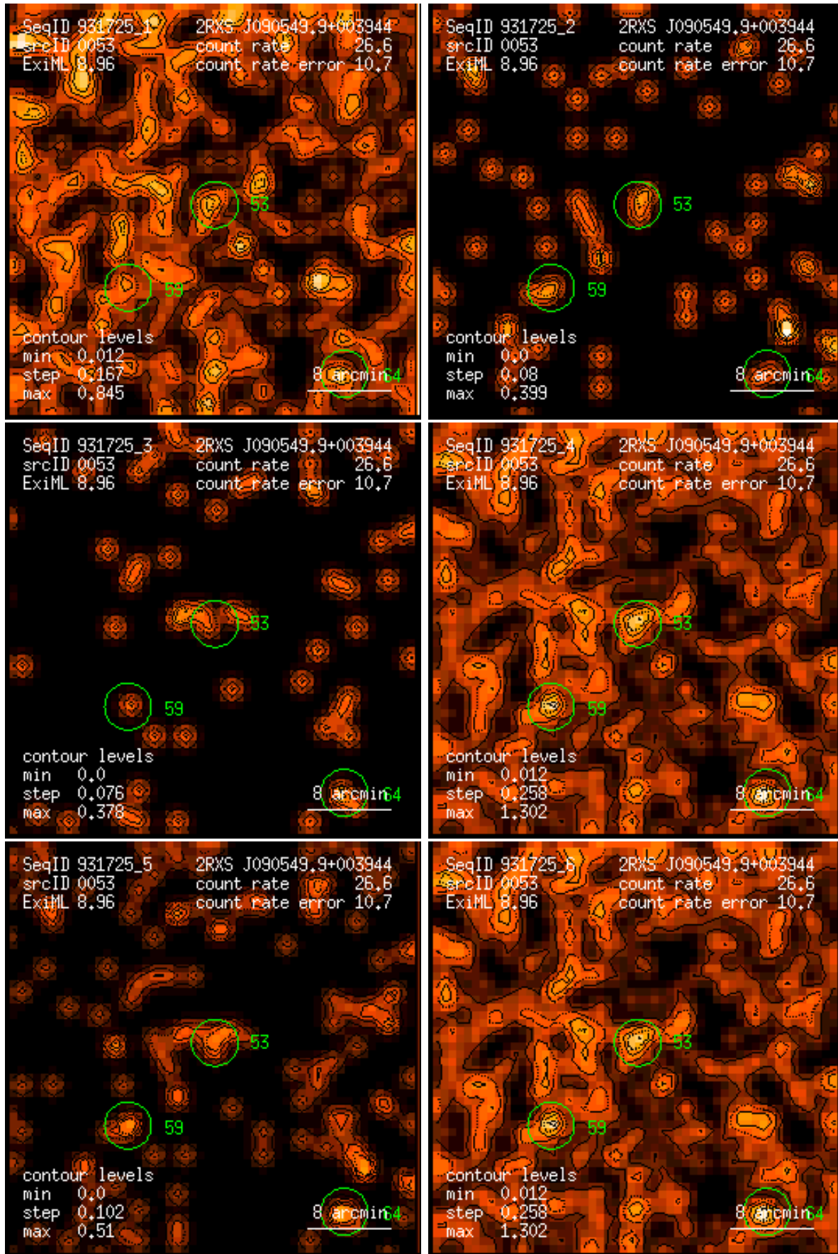
Figure 53: RASS 931725: detection 0053: band rate images, Gaussian filter: (1) PSPC channels 11 – 41, (2) 52 – 90, (3) 91 – 201, (4) 11 – 235, (5) 52 – 201, (6) 11 – 201. Broad band rates in counts/ks. Band rate contour levels in counts/ks/arcmin 2 .
