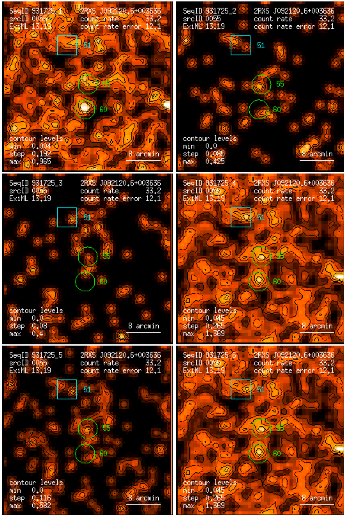
Figure 55: RASS 931725: detection 0055: band rate images, Gaussian filter: (1) PSPC channels 11 – 41, (2) 52 – 90, (3) 91 – 201, (4) 11 – 235, (5) 52 – 201, (6) 11 – 201. Broad band rates in counts/ks. Band rate contour levels in counts/ks/arcmin 2 .
