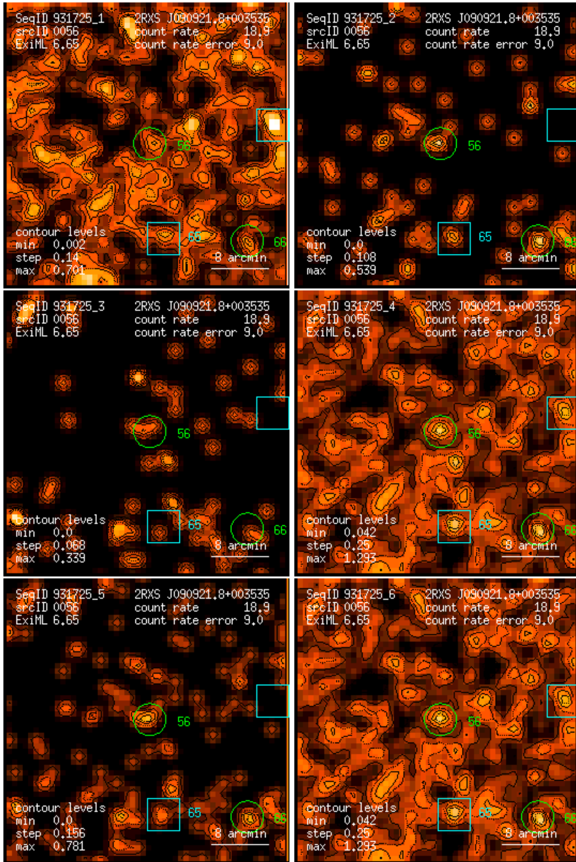
Figure 56: RASS 931725: detection 0056: band rate images, Gaussian filter: (1) PSPC channels 11 – 41, (2) 52 – 90, (3) 91 – 201, (4) 11 – 235, (5) 52 – 201, (6) 11 – 201. Broad band rates in counts/ks. Band rate contour levels in counts/ks/arcmin 2 .
