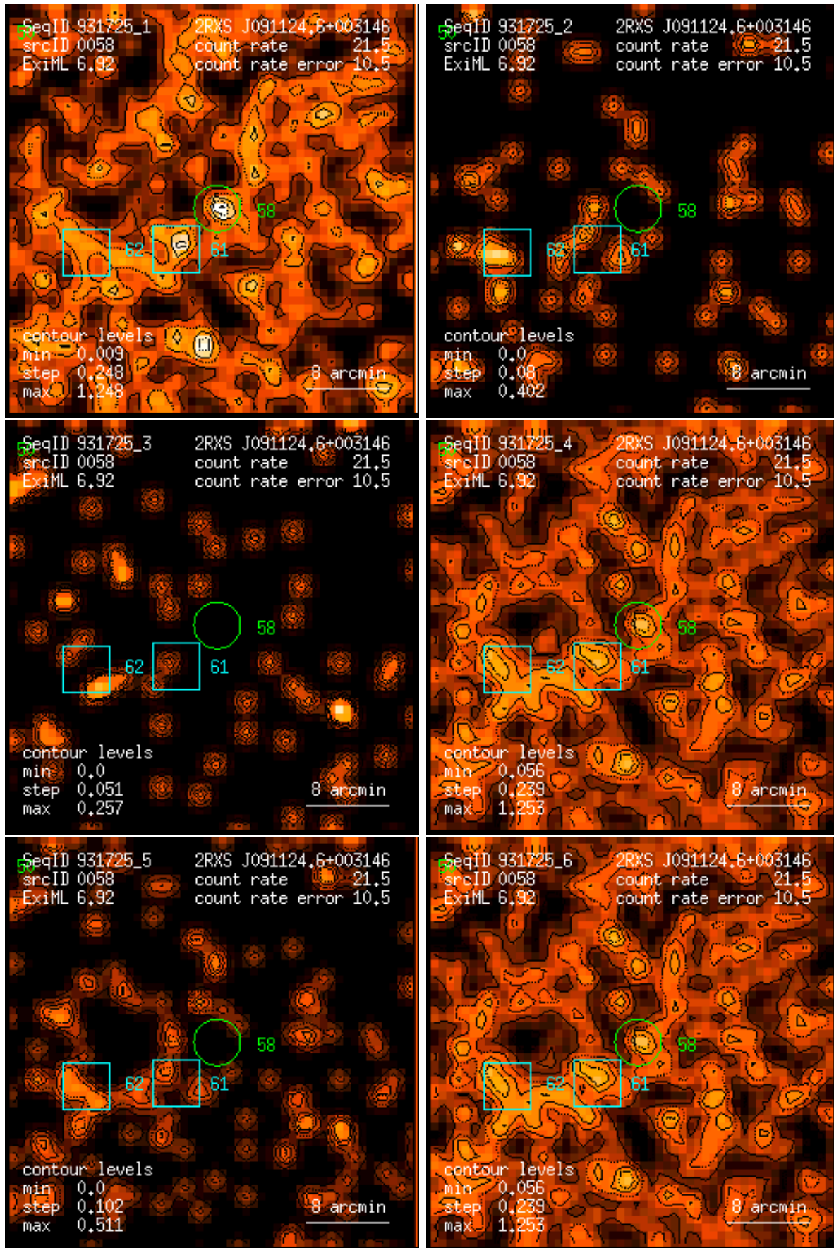
Figure 58: RASS 931725: detection 0058: band rate images, Gaussian filter: (1) PSPC channels 11 – 41, (2) 52 – 90, (3) 91 – 201, (4) 11 – 235, (5) 52 – 201, (6) 11 – 201. Broad band rates in counts/ks. Band rate contour levels in counts/ks/arcmin 2 .
