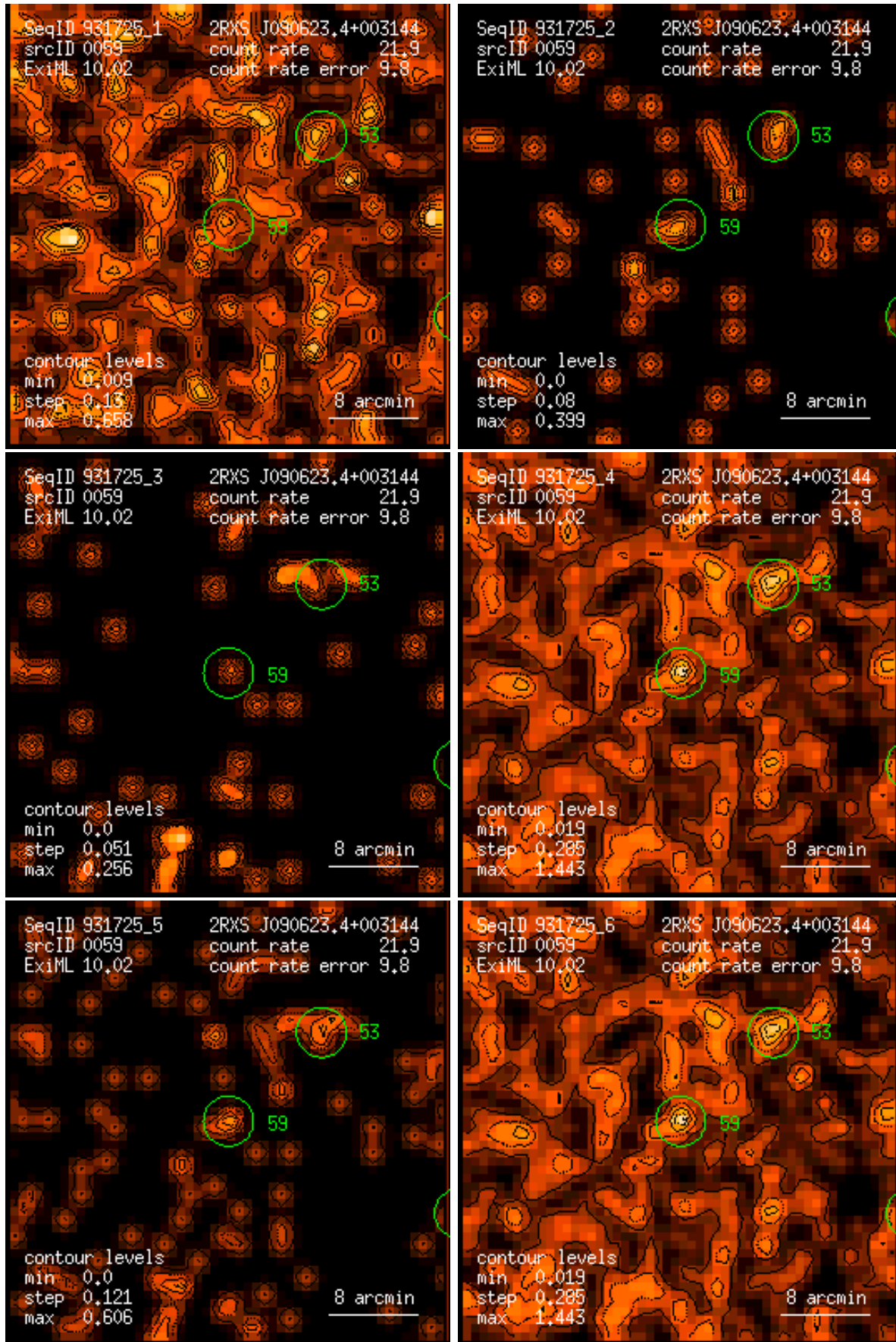
Figure 59: RASS 931725: detection 0059: band rate images, Gaussian filter: (1) PSPC channels 11 – 41, (2) 52 – 90, (3) 91 – 201, (4) 11 – 235, (5) 52 – 201, (6) 11 – 201. Broad band rates in counts/ks. Band rate contour levels in counts/ks/arcmin 2 .
