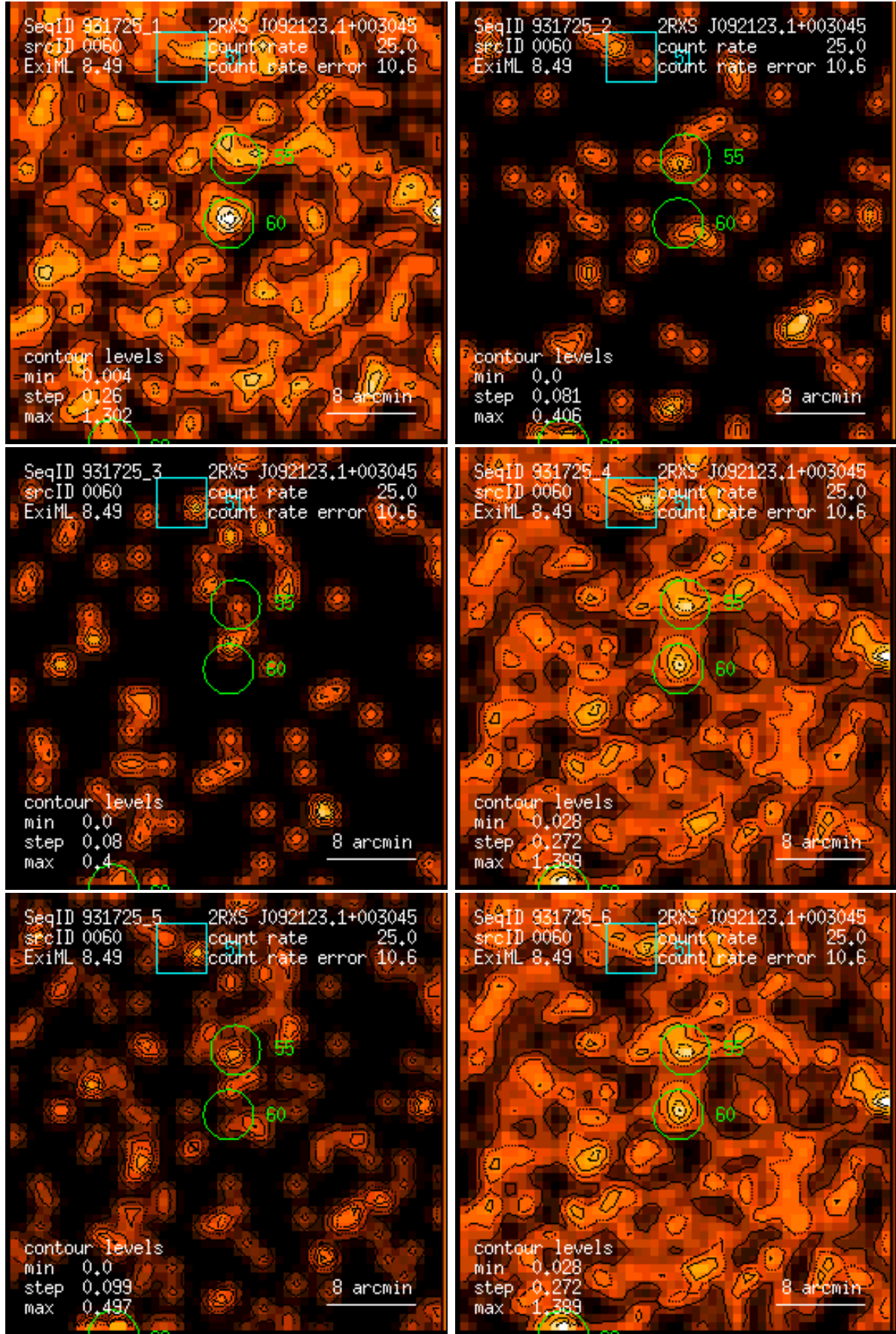
Figure 60: RASS 931725: detection 0060: band rate images, Gaussian filter: (1) PSPC channels 11 – 41, (2) 52 – 90, (3) 91 – 201, (4) 11 – 235, (5) 52 – 201, (6) 11 – 201. Broad band rates in counts/ks. Band rate contour levels in counts/ks/arcmin 2 .
