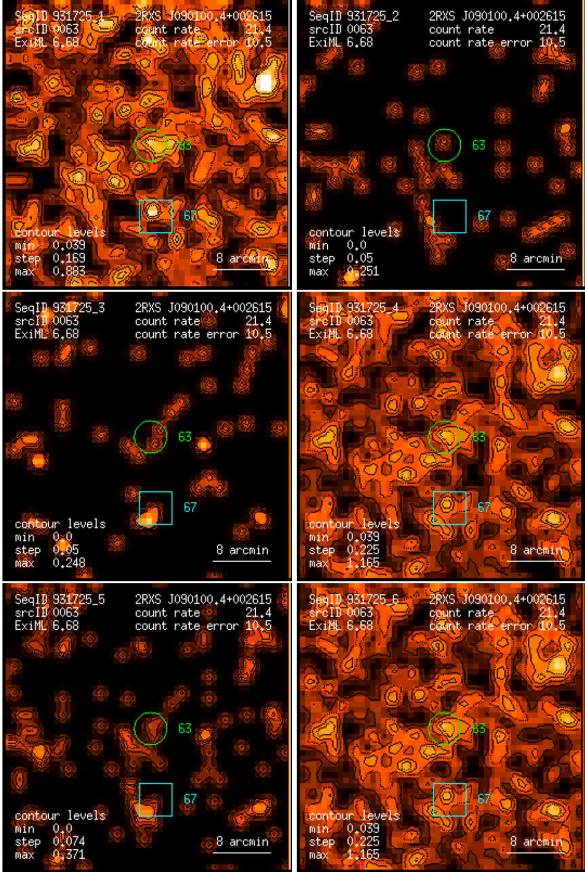
Figure 63: RASS 931725: detection 0063: band rate images, Gaussian filter: (1) PSPC channels 11 – 41, (2) 52 – 90, (3) 91 – 201, (4) 11 – 235, (5) 52 – 201, (6) 11 – 201. Broad band rates in counts/ks. Band rate contour levels in counts/ks/arcmin 2 .
