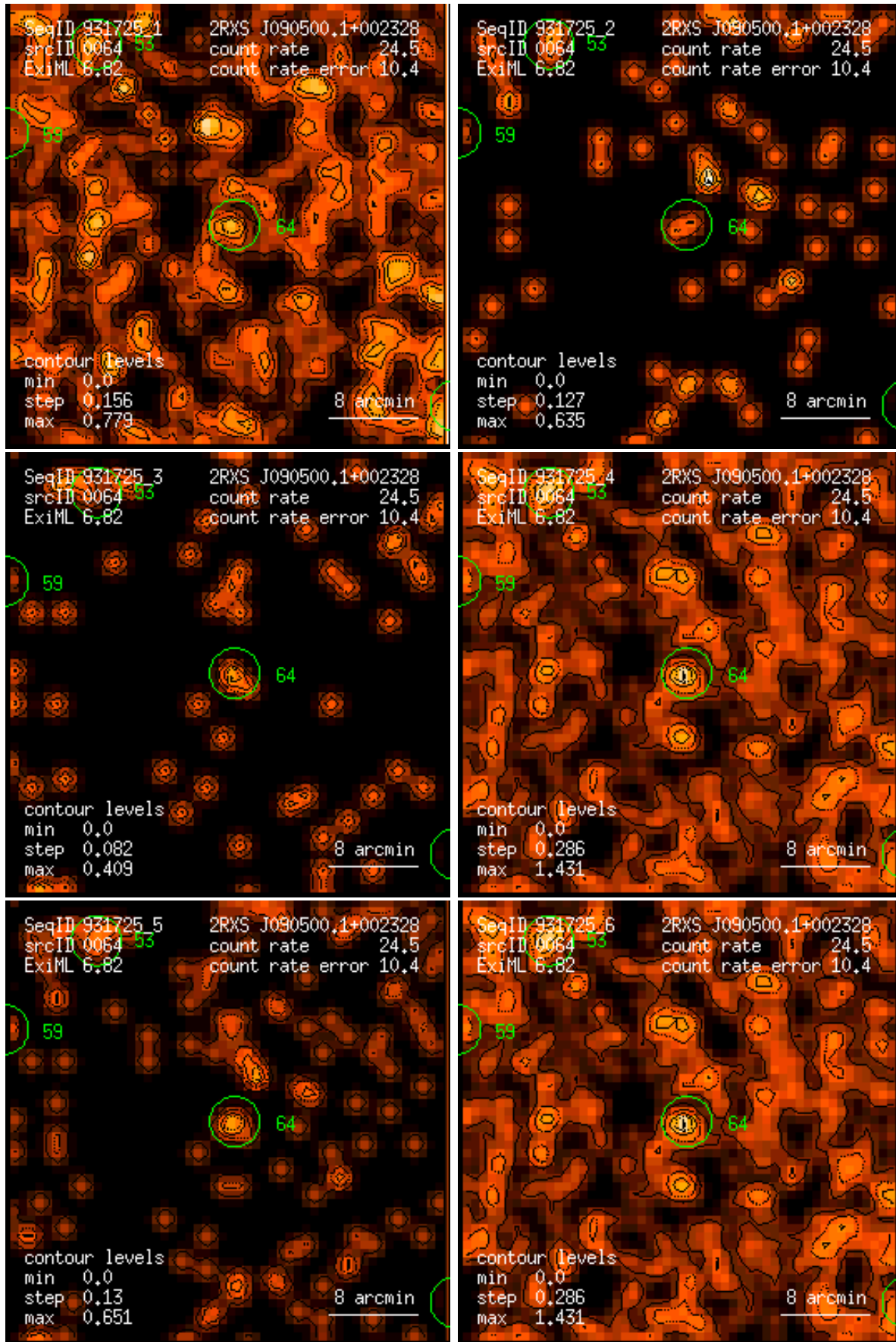
Figure 64: RASS 931725: detection 0064: band rate images, Gaussian filter: (1) PSPC channels 11 – 41, (2) 52 – 90, (3) 91 – 201, (4) 11 – 235, (5) 52 – 201, (6) 11 – 201. Broad band rates in counts/ks. Band rate contour levels in counts/ks/arcmin 2 .
