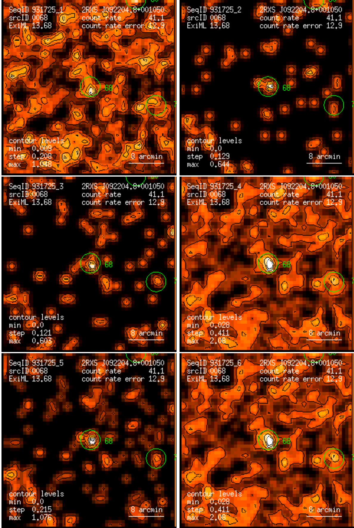
Figure 68: RASS 931725: detection 0068: band rate images, Gaussian filter: (1) PSPC channels 11 – 41, (2) 52 – 90, (3) 91 – 201, (4) 11 – 235, (5) 52 – 201, (6) 11 – 201. Broad band rates in counts/ks. Band rate contour levels in counts/ks/arcmin 2 .
