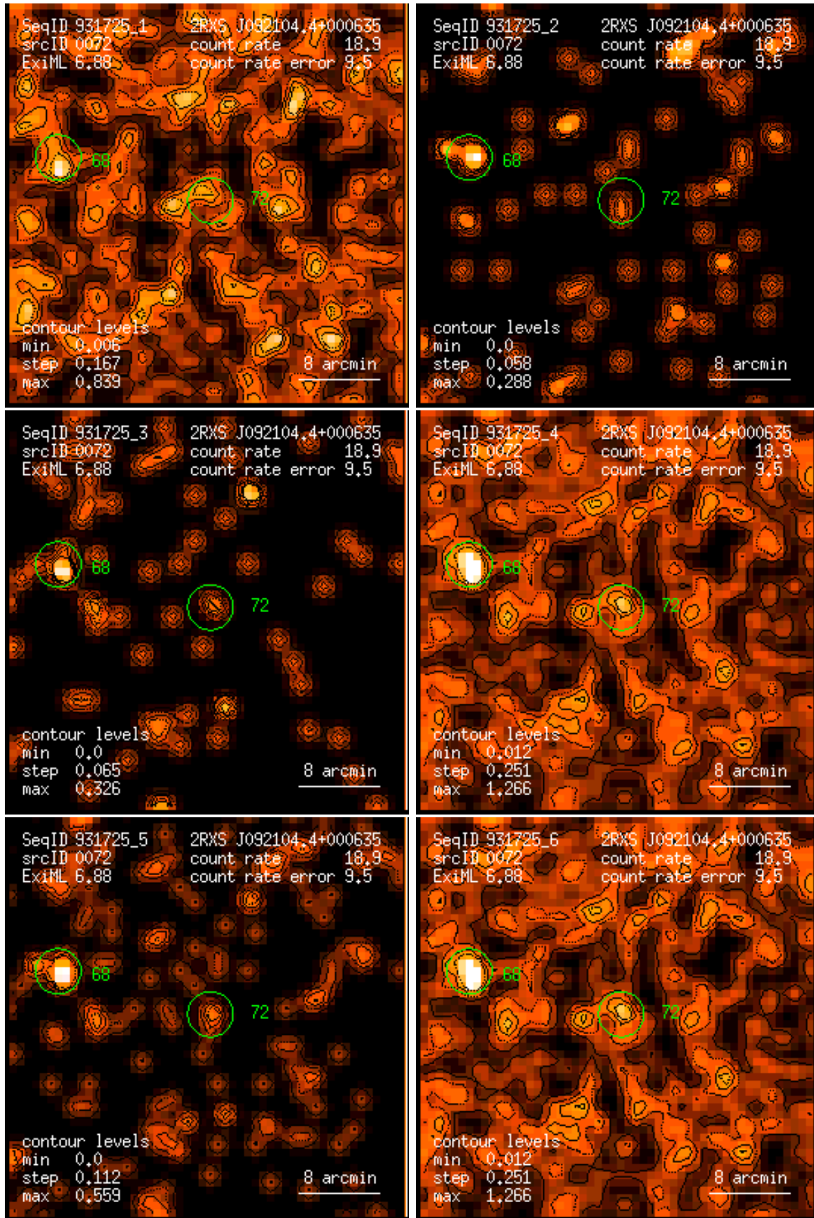
Figure 72: RASS 931725: detection 0072: band rate images, Gaussian filter: (1) PSPC channels 11 – 41, (2) 52 – 90, (3) 91 – 201, (4) 11 – 235, (5) 52 – 201, (6) 11 – 201. Broad band rates in counts/ks. Band rate contour levels in counts/ks/arcmin 2 .
