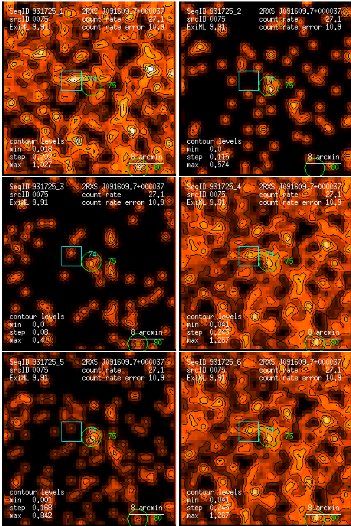
Figure 75: RASS 931725: detection 0075: band rate images, Gaussian filter: (1) PSPC channels 11 – 41, (2) 52 – 90, (3) 91 – 201, (4) 11 – 235, (5) 52 – 201, (6) 11 – 201. Broad band rates in counts/ks. Band rate contour levels in counts/ks/arcmin 2 .
