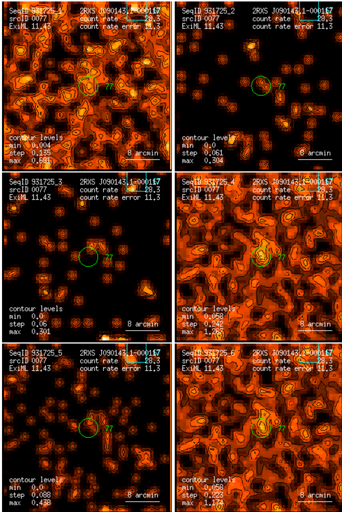
Figure 77: RASS 931725: detection 0077: band rate images, Gaussian filter: (1) PSPC channels 11 – 41, (2) 52 – 90, (3) 91 – 201, (4) 11 – 235, (5) 52 – 201, (6) 11 – 201. Broad band rates in counts/ks. Band rate contour levels in counts/ks/arcmin 2 .
