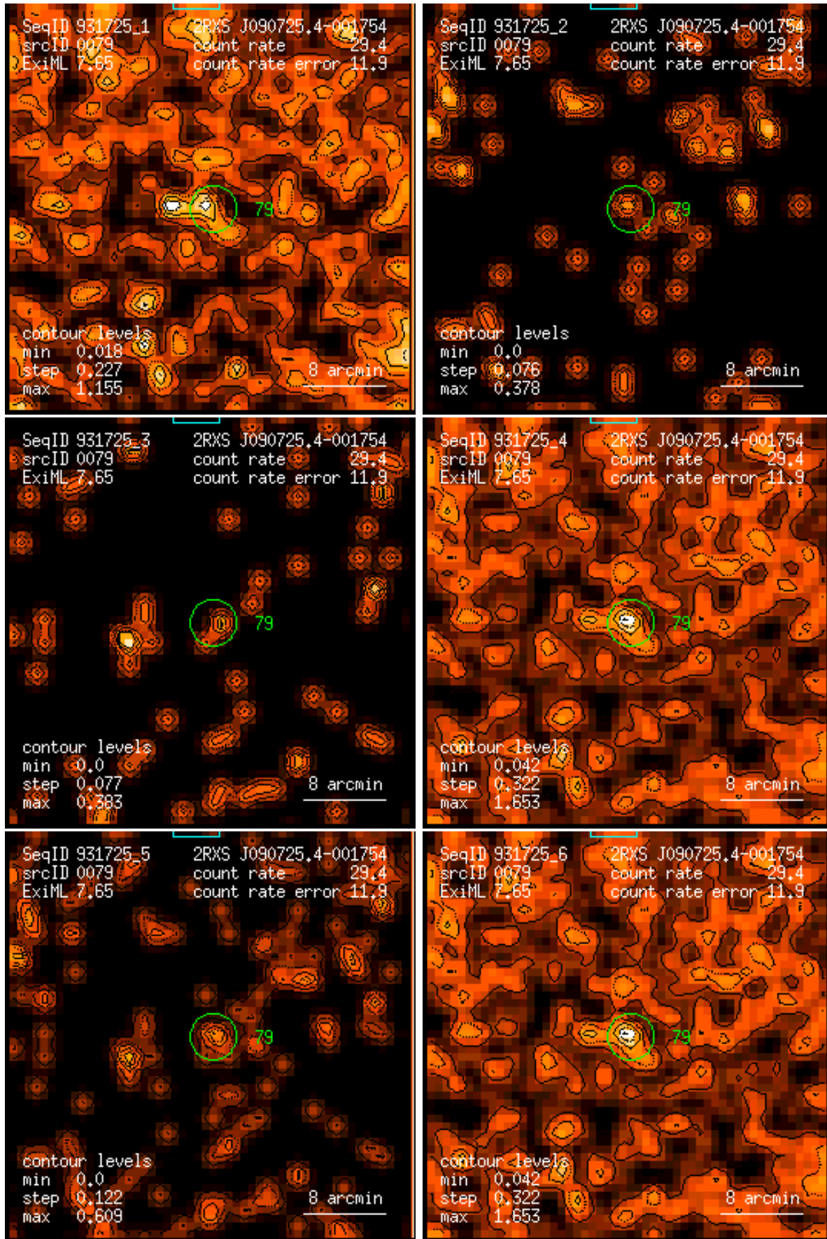
Figure 79: RASS 931725: detection 0079: band rate images, Gaussian filter: (1) PSPC channels 11 – 41, (2) 52 – 90, (3) 91 – 201, (4) 11 – 235, (5) 52 – 201, (6) 11 – 201. Broad band rates in counts/ks. Band rate contour levels in counts/ks/arcmin 2 .
