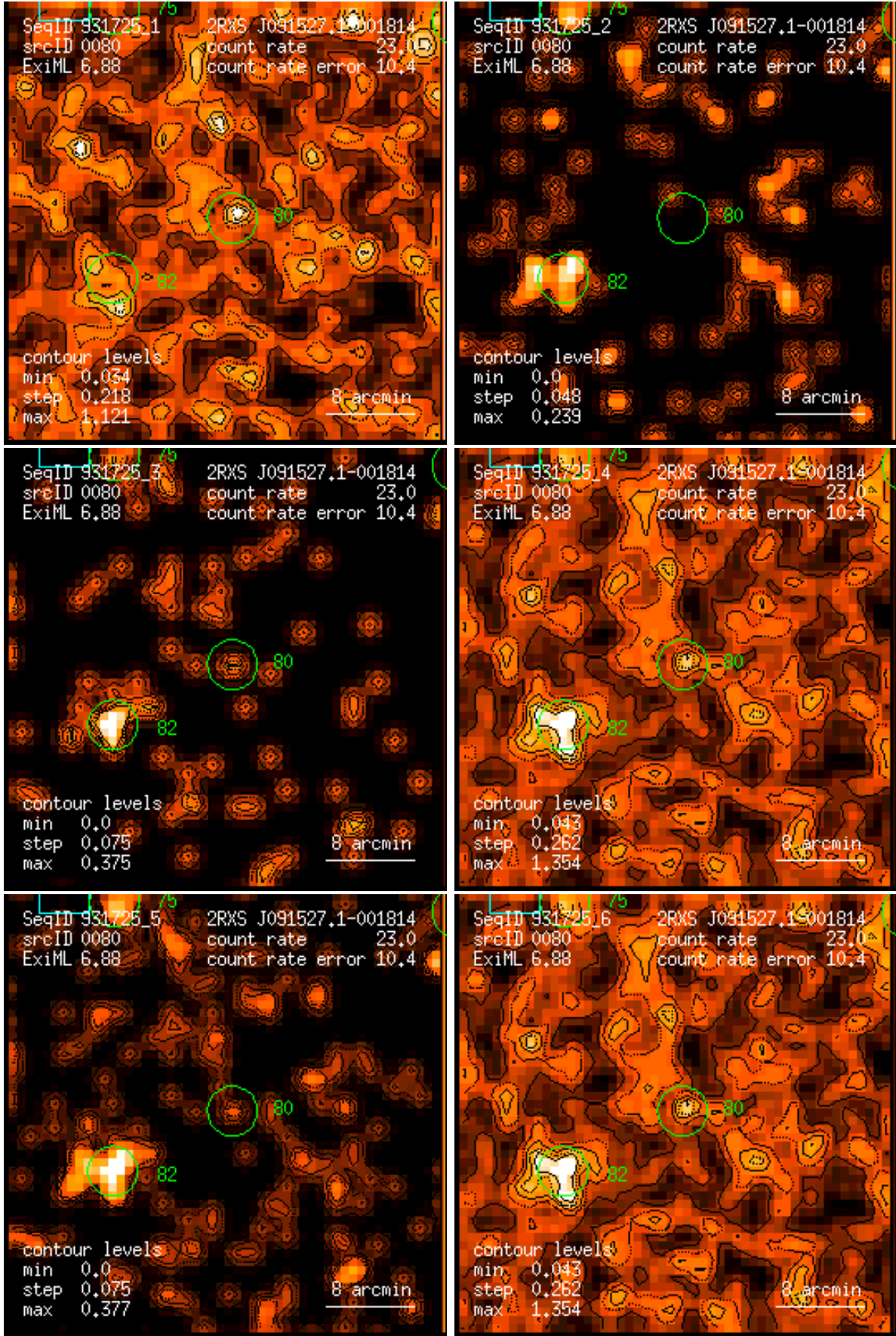
Figure 80: RASS 931725: detection 0080: band rate images, Gaussian filter: (1) PSPC channels 11 – 41, (2) 52 – 90, (3) 91 – 201, (4) 11 – 235, (5) 52 – 201, (6) 11 – 201. Broad band rates in counts/ks. Band rate contour levels in counts/ks/arcmin 2 .
