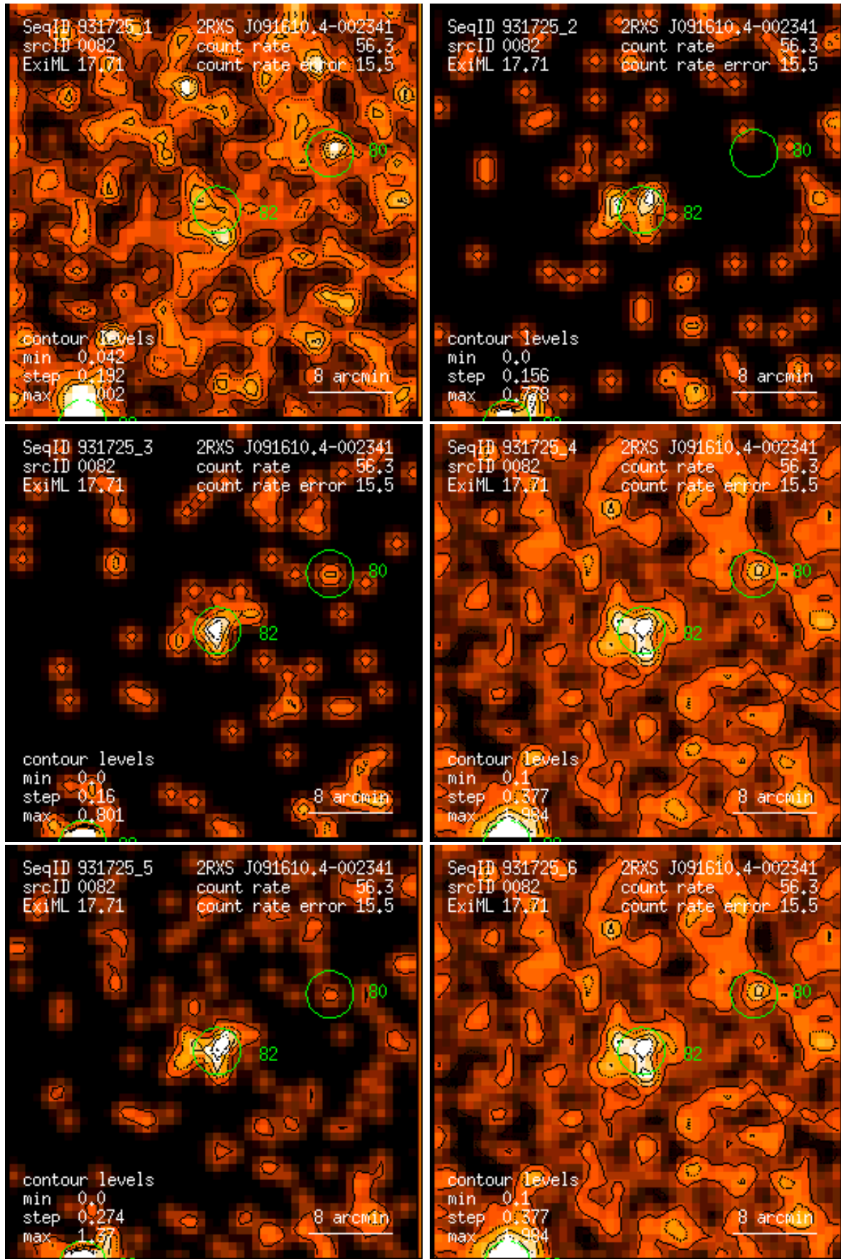
Figure 82: RASS 931725: detection 0082: band rate images, Gaussian filter: (1) PSPC channels 11 – 41, (2) 52 – 90, (3) 91 – 201, (4) 11 – 235, (5) 52 – 201, (6) 11 – 201. Broad band rates in counts/ks. Band rate contour levels in counts/ks/arcmin 2 .
