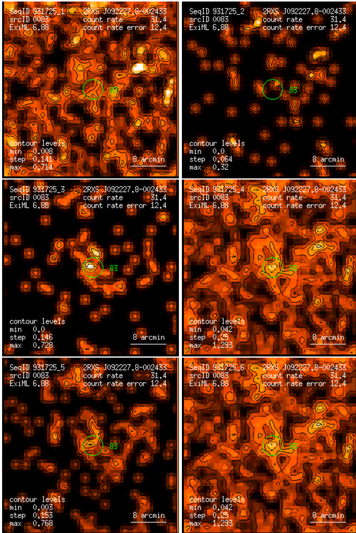
Figure 83: RASS 931725: detection 0083: band rate images, Gaussian filter: (1) PSPC channels 11 – 41, (2) 52 – 90, (3) 91 – 201, (4) 11 – 235, (5) 52 – 201, (6) 11 – 201. Broad band rates in counts/ks. Band rate contour levels in counts/ks/arcmin 2 .
