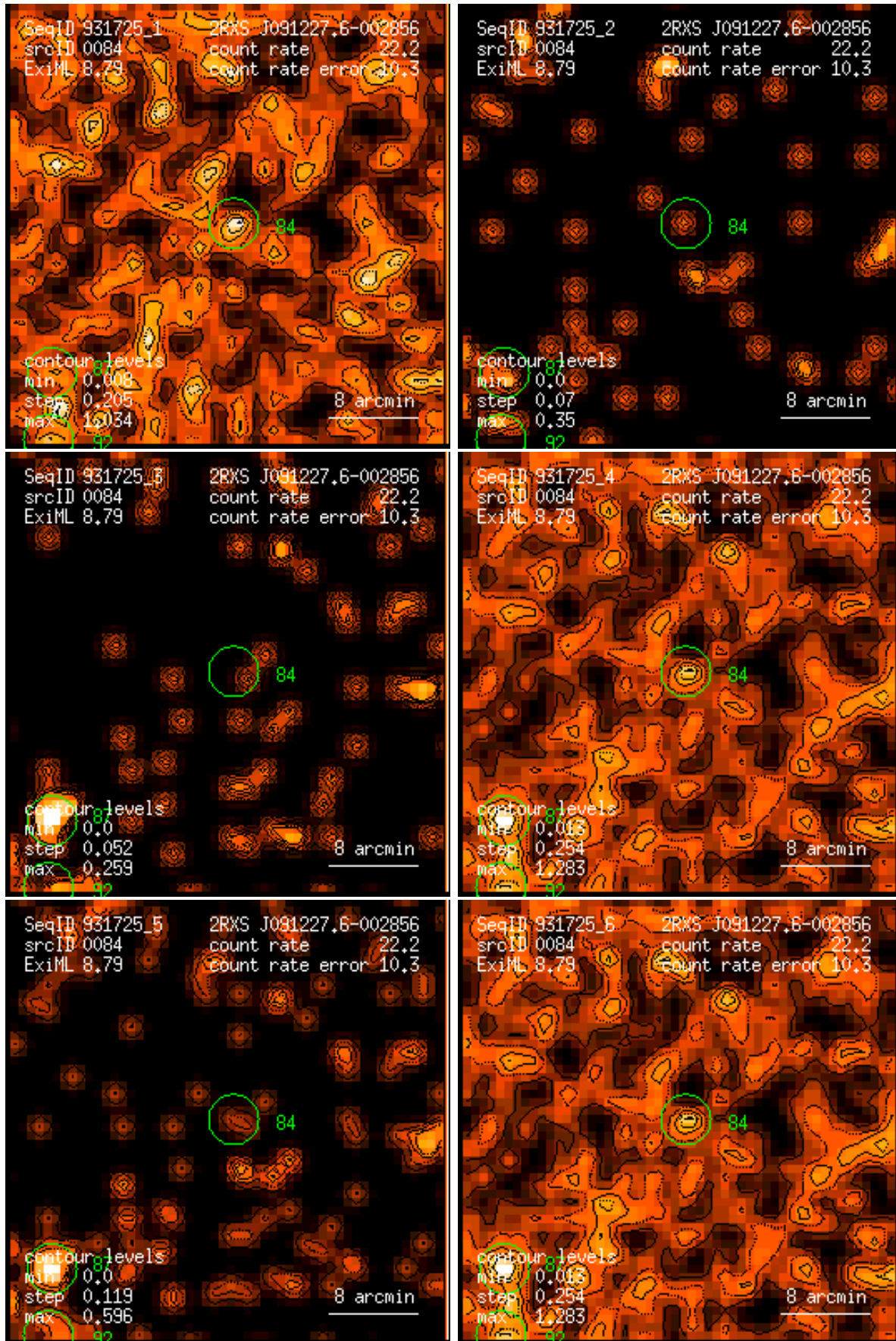
Figure 84: RASS 931725: detection 0084: band rate images, Gaussian filter: (1) PSPC channels 11 – 41, (2) 52 – 90, (3) 91 – 201, (4) 11 – 235, (5) 52 – 201, (6) 11 – 201. Broad band rates in counts/ks. Band rate contour levels in counts/ks/arcmin 2 .
