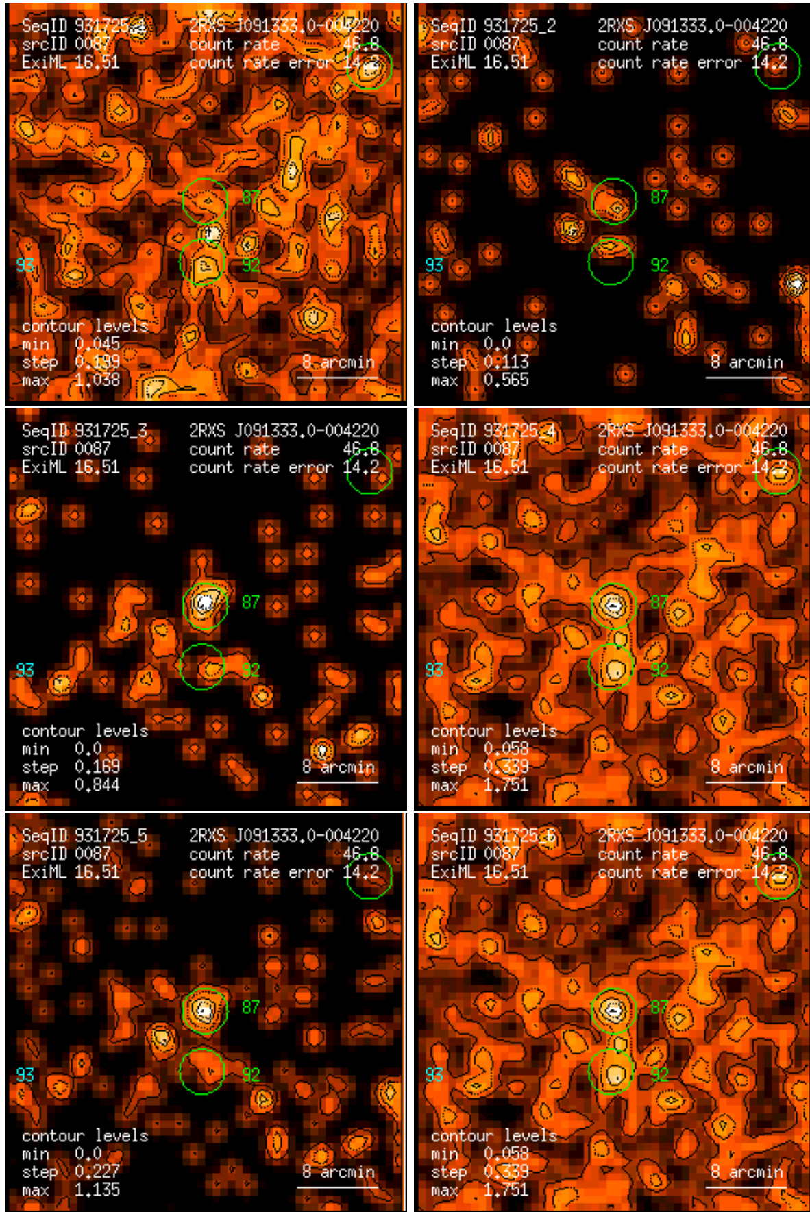
Figure 87: RASS 931725: detection 0087: band rate images, Gaussian filter: (1) PSPC channels 11 – 41, (2) 52 – 90, (3) 91 – 201, (4) 11 – 235, (5) 52 – 201, (6) 11 – 201. Broad band rates in counts/ks. Band rate contour levels in counts/ks/arcmin 2 .
