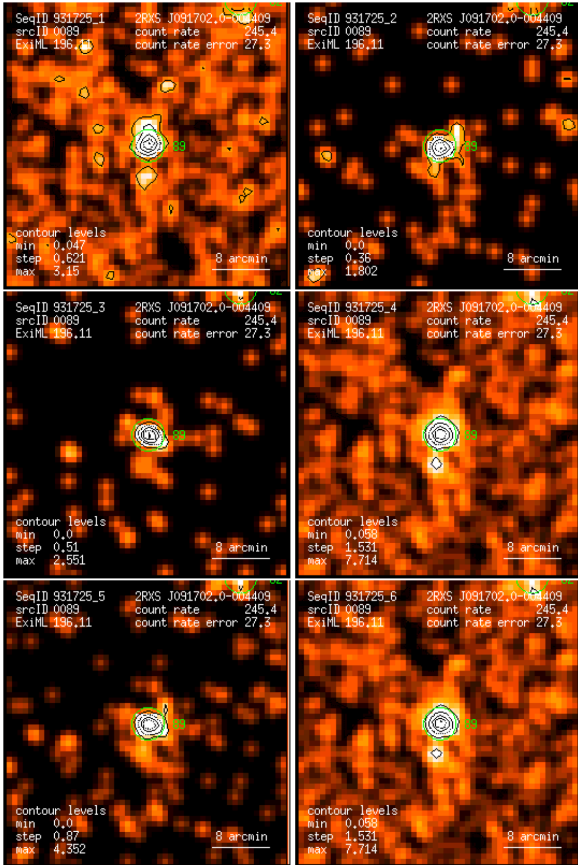
Figure 89: RASS 931725: detection 0089: band rate images, Gaussian filter: (1) PSPC channels 11 – 41, (2) 52 – 90, (3) 91 – 201, (4) 11 – 235, (5) 52 – 201, (6) 11 – 201. Broad band rates in counts/ks. Band rate contour levels in counts/ks/arcmin 2 .
