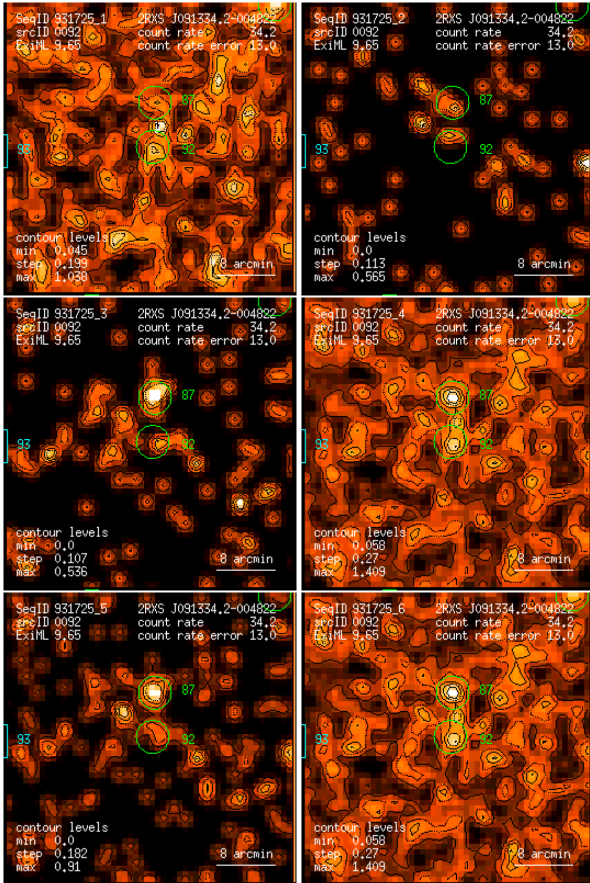
Figure 92: RASS 931725: detection 0092: band rate images, Gaussian filter: (1) PSPC channels 11 – 41, (2) 52 – 90, (3) 91 – 201, (4) 11 – 235, (5) 52 – 201, (6) 11 – 201. Broad band rates in counts/ks. Band rate contour levels in counts/ks/arcmin 2 .
