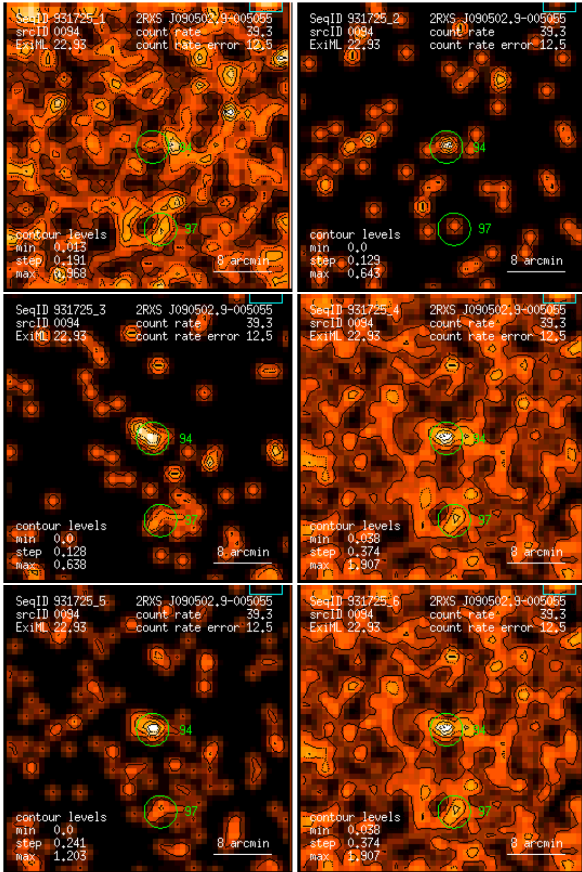
Figure 94: RASS 931725: detection 0094: band rate images, Gaussian filter: (1) PSPC channels 11 – 41, (2) 52 – 90, (3) 91 – 201, (4) 11 – 235, (5) 52 – 201, (6) 11 – 201. Broad band rates in counts/ks. Band rate contour levels in counts/ks/arcmin 2 .
