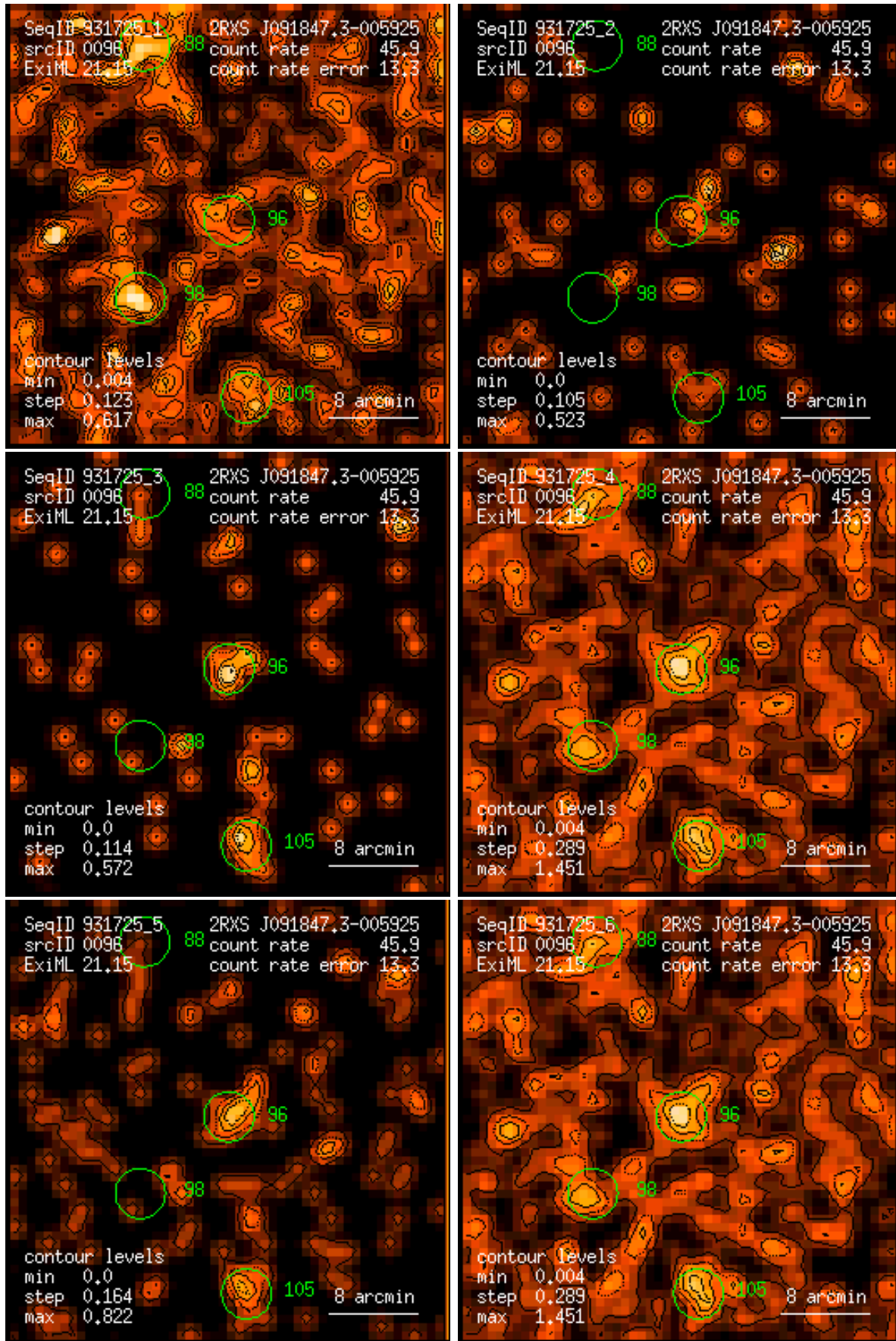
Figure 96: RASS 931725: detection 0096: band rate images, Gaussian filter: (1) PSPC channels 11 – 41, (2) 52 – 90, (3) 91 – 201, (4) 11 – 235, (5) 52 – 201, (6) 11 – 201. Broad band rates in counts/ks. Band rate contour levels in counts/ks/arcmin 2 .
